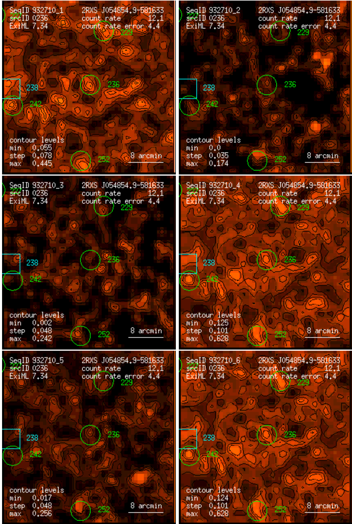
Figure 236: RASS 932710: detection 0236: band rate images, Gaussian filter: (1) PSPC channels 11 – 41, (2) 52 – 90, (3) 91 – 201, (4) 11 – 235, (5) 52 – 201, (6) 11 – 201. Broad band rates in counts/ks. Band rate contour levels in counts/ks/arcmin 2 .
