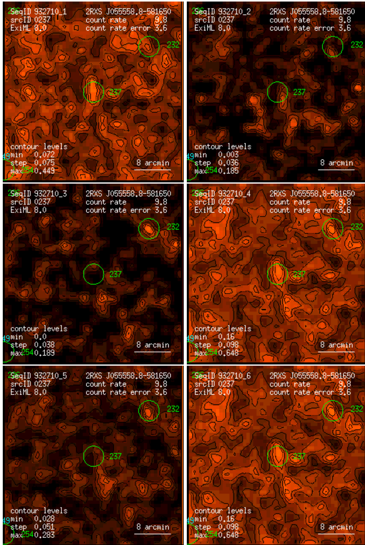
Figure 237: RASS 932710: detection 0237: band rate images, Gaussian filter: (1) PSPC channels 11 – 41, (2) 52 – 90, (3) 91 – 201, (4) 11 – 235, (5) 52 – 201, (6) 11 – 201. Broad band rates in counts/ks. Band rate contour levels in counts/ks/arcmin 2 .
