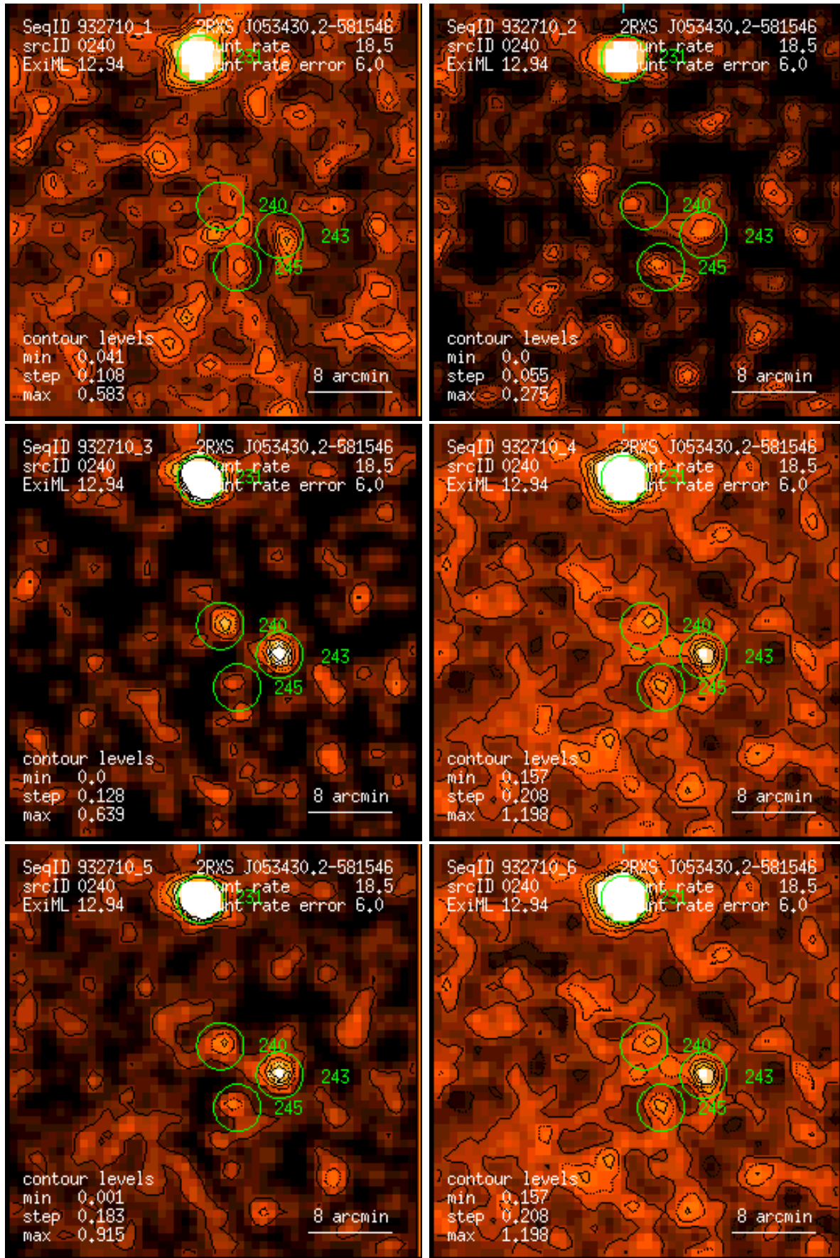
Figure 240: RASS 932710: detection 0240: band rate images, Gaussian filter: (1) PSPC channels 11 – 41, (2) 52 – 90, (3) 91 – 201, (4) 11 – 235, (5) 52 – 201, (6) 11 – 201. Broad band rates in counts/ks. Band rate contour levels in counts/ks/arcmin 2 .
