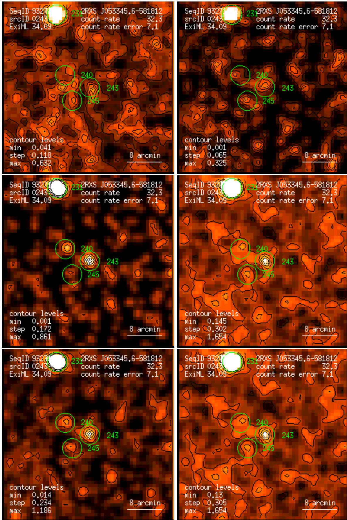
Figure 243: RASS 932710: detection 0243: band rate images, Gaussian filter: (1) PSPC channels 11 – 41, (2) 52 – 90, (3) 91 – 201, (4) 11 – 235, (5) 52 – 201, (6) 11 – 201. Broad band rates in counts/ks. Band rate contour levels in counts/ks/arcmin 2 .
