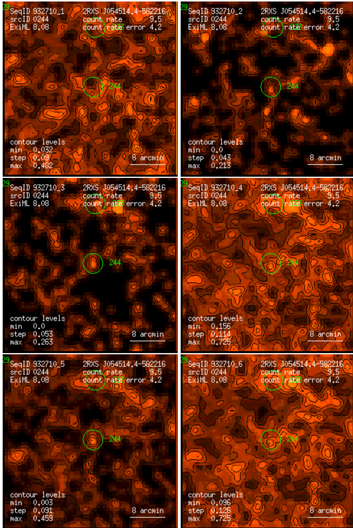
Figure 244: RASS 932710: detection 0244: band rate images, Gaussian filter: (1) PSPC channels 11 – 41, (2) 52 – 90, (3) 91 – 201, (4) 11 – 235, (5) 52 – 201, (6) 11 – 201. Broad band rates in counts/ks. Band rate contour levels in counts/ks/arcmin 2 .
