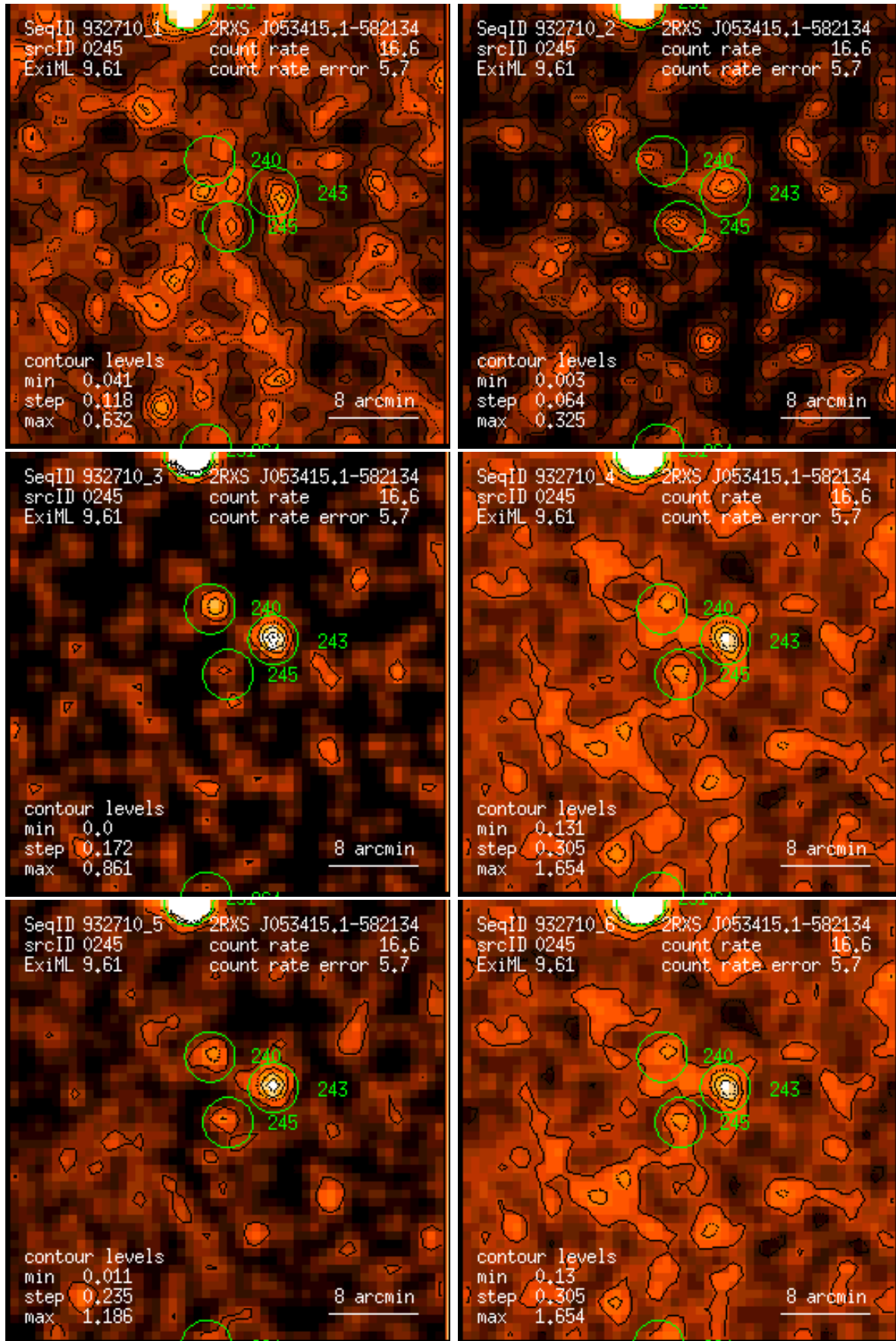
Figure 245: RASS 932710: detection 0245: band rate images, Gaussian filter: (1) PSPC channels 11 – 41, (2) 52 – 90, (3) 91 – 201, (4) 11 – 235, (5) 52 – 201, (6) 11 – 201. Broad band rates in counts/ks. Band rate contour levels in counts/ks/arcmin 2 .
