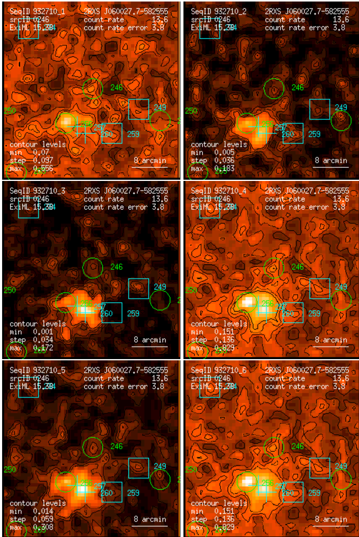
Figure 246: RASS 932710: detection 0246: band rate images, Gaussian filter: (1) PSPC channels 11 – 41, (2) 52 – 90, (3) 91 – 201, (4) 11 – 235, (5) 52 – 201, (6) 11 – 201. Broad band rates in counts/ks. Band rate contour levels in counts/ks/arcmin 2 .
