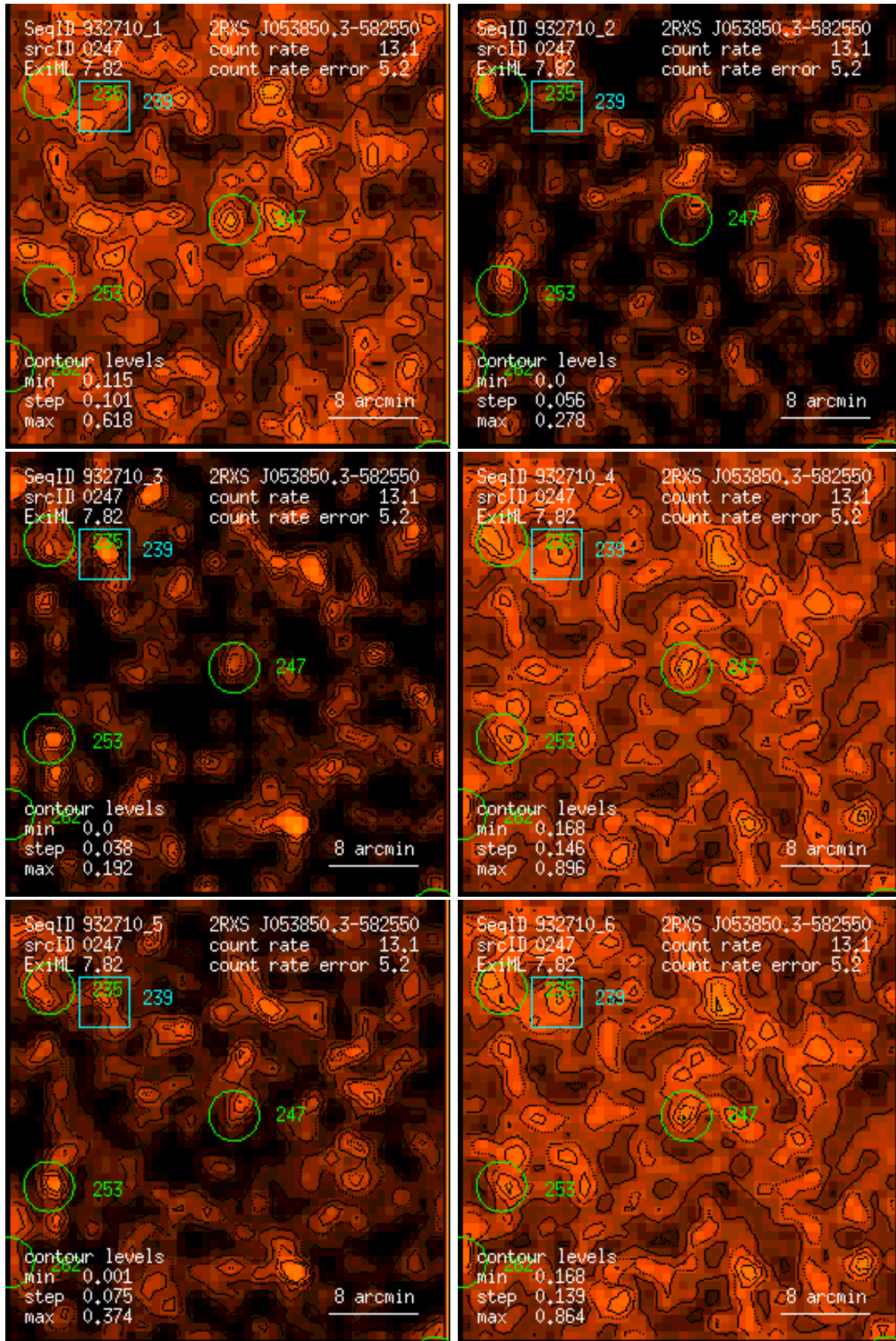
Figure 247: RASS 932710: detection 0247: band rate images, Gaussian filter: (1) PSPC channels 11 – 41, (2) 52 – 90, (3) 91 – 201, (4) 11 – 235, (5) 52 – 201, (6) 11 – 201. Broad band rates in counts/ks. Band rate contour levels in counts/ks/arcmin 2 .
