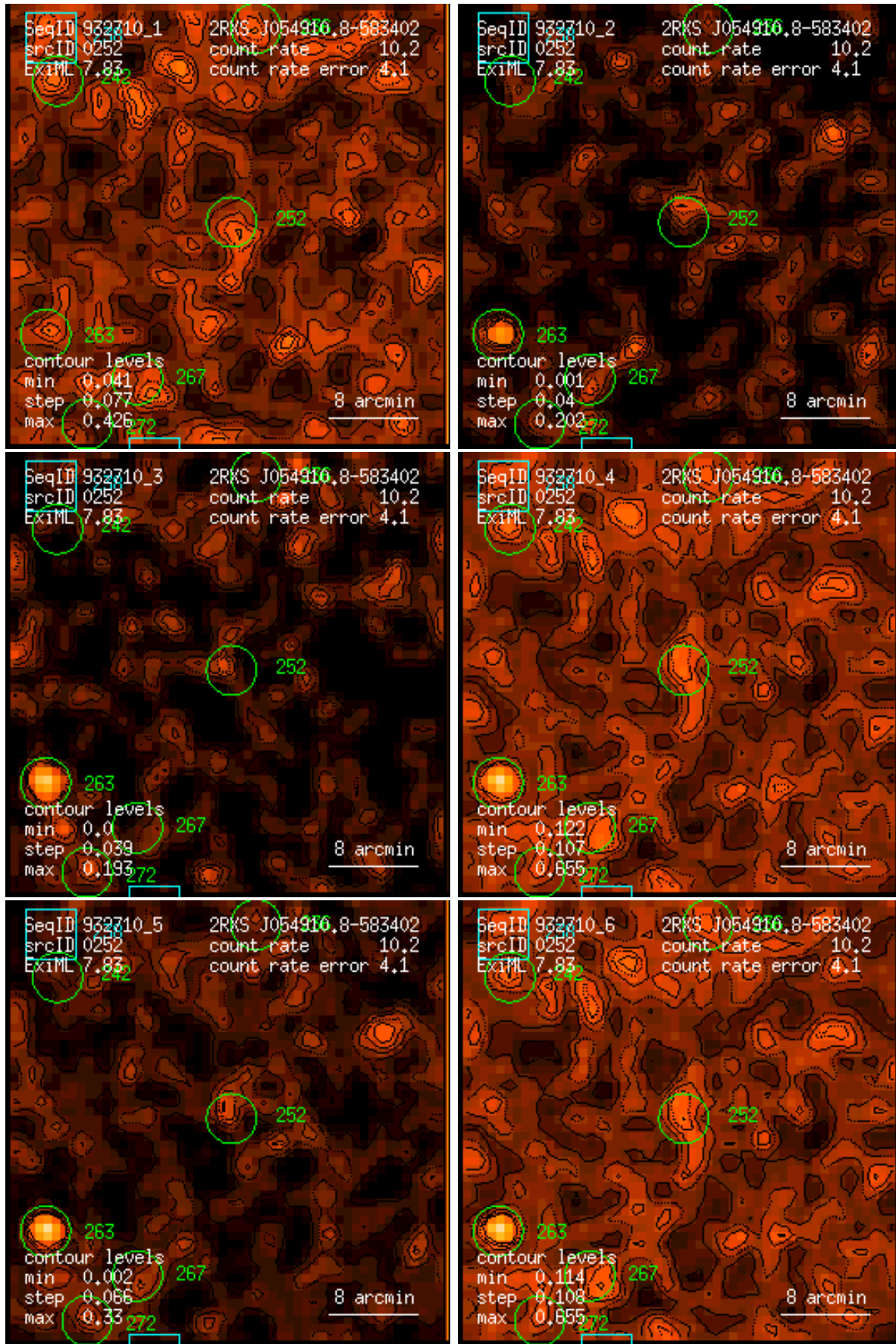
Figure 252: RASS 932710: detection 0252: band rate images, Gaussian filter: (1) PSPC channels 11 – 41, (2) 52 – 90, (3) 91 – 201, (4) 11 – 235, (5) 52 – 201, (6) 11 – 201. Broad band rates in counts/ks. Band rate contour levels in counts/ks/arcmin 2 .
