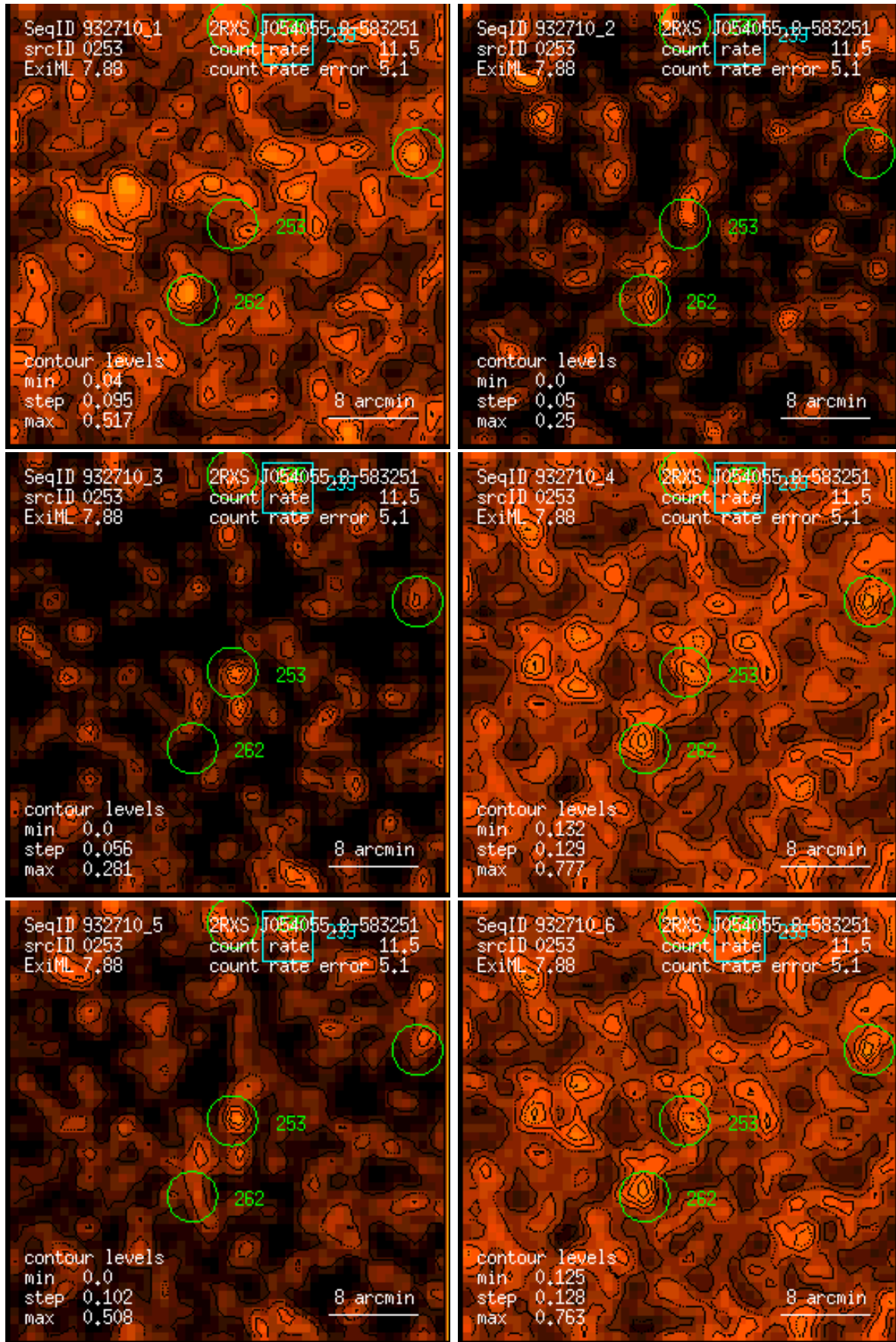
Figure 253: RASS 932710: detection 0253: band rate images, Gaussian filter: (1) PSPC channels 11 – 41, (2) 52 – 90, (3) 91 – 201, (4) 11 – 235, (5) 52 – 201, (6) 11 – 201. Broad band rates in counts/ks. Band rate contour levels in counts/ks/arcmin 2 .
