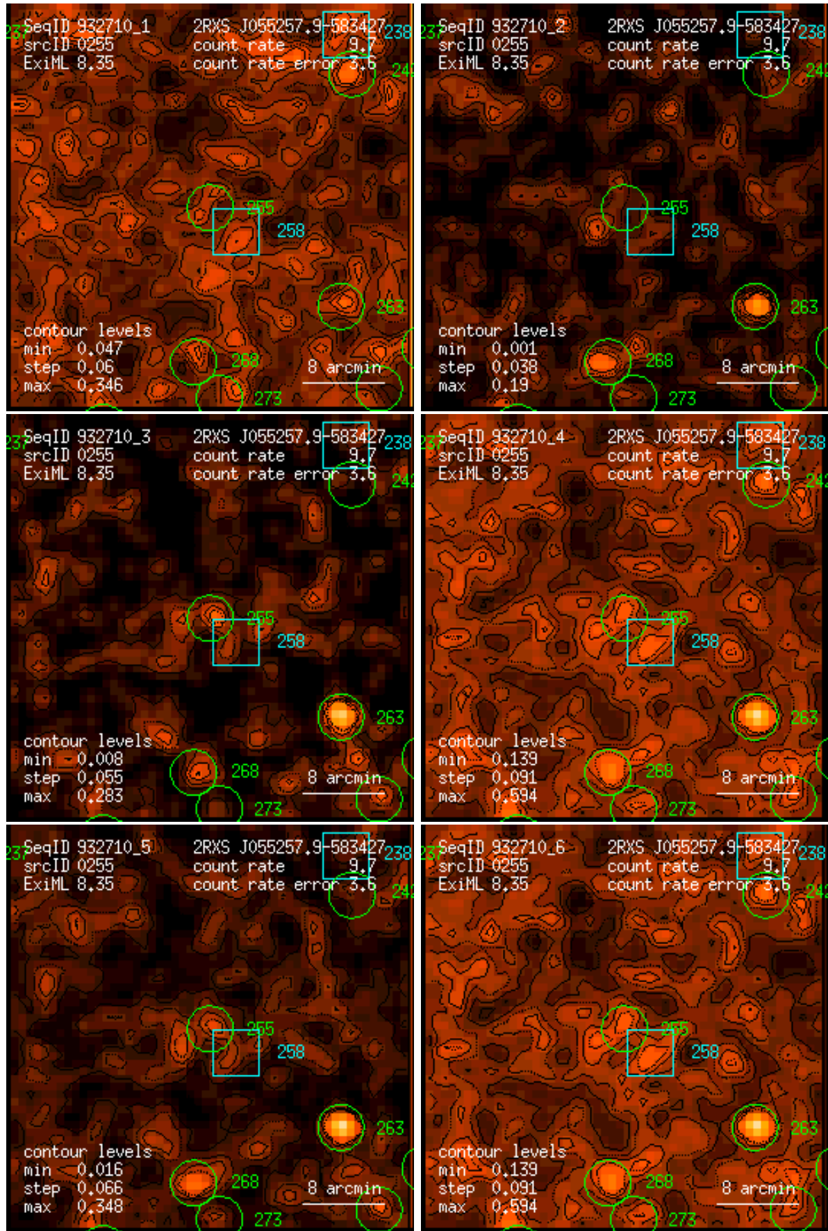
Figure 255: RASS 932710: detection 0255: band rate images, Gaussian filter: (1) PSPC channels 11 – 41, (2) 52 – 90, (3) 91 – 201, (4) 11 – 235, (5) 52 – 201, (6) 11 – 201. Broad band rates in counts/ks. Band rate contour levels in counts/ks/arcmin 2 .
