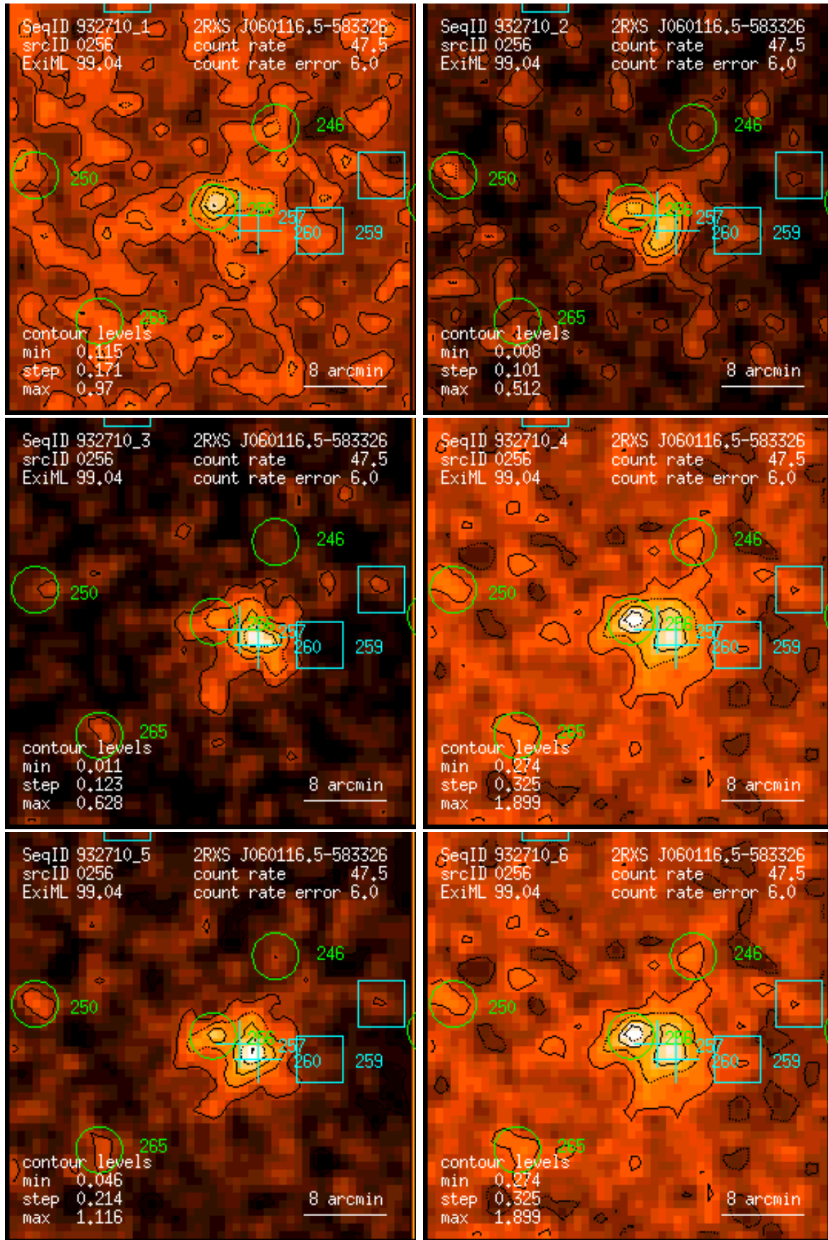
Figure 256: RASS 932710: detection 0256: band rate images, Gaussian filter: (1) PSPC channels 11 – 41, (2) 52 – 90, (3) 91 – 201, (4) 11 – 235, (5) 52 – 201, (6) 11 – 201. Broad band rates in counts/ks. Band rate contour levels in counts/ks/arcmin 2 .
