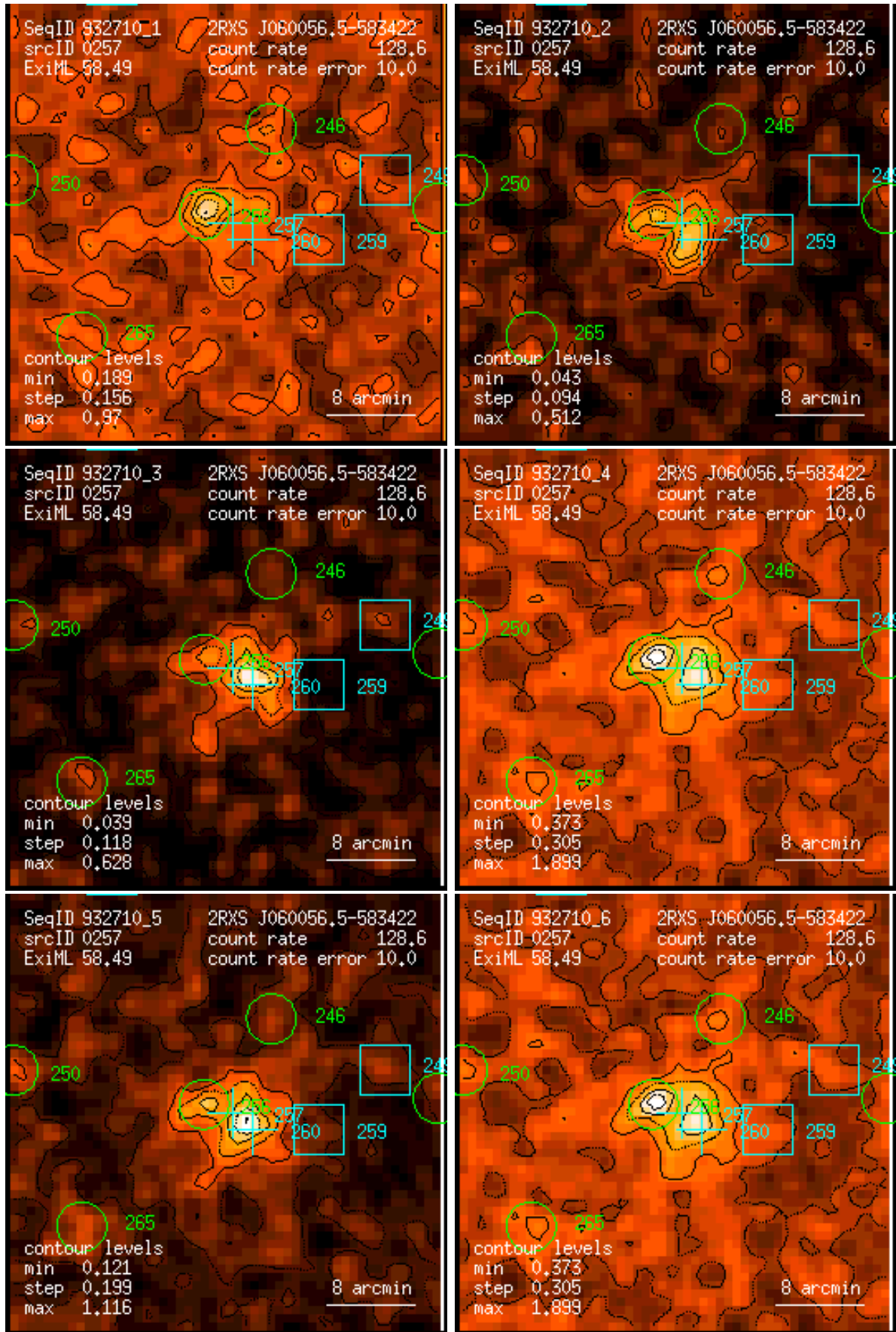
Figure 257: RASS 932710: detection 0257: band rate images, Gaussian filter: (1) PSPC channels 11 – 41, (2) 52 – 90, (3) 91 – 201, (4) 11 – 235, (5) 52 – 201, (6) 11 – 201. Broad band rates in counts/ks. Band rate contour levels in counts/ks/arcmin 2 .
