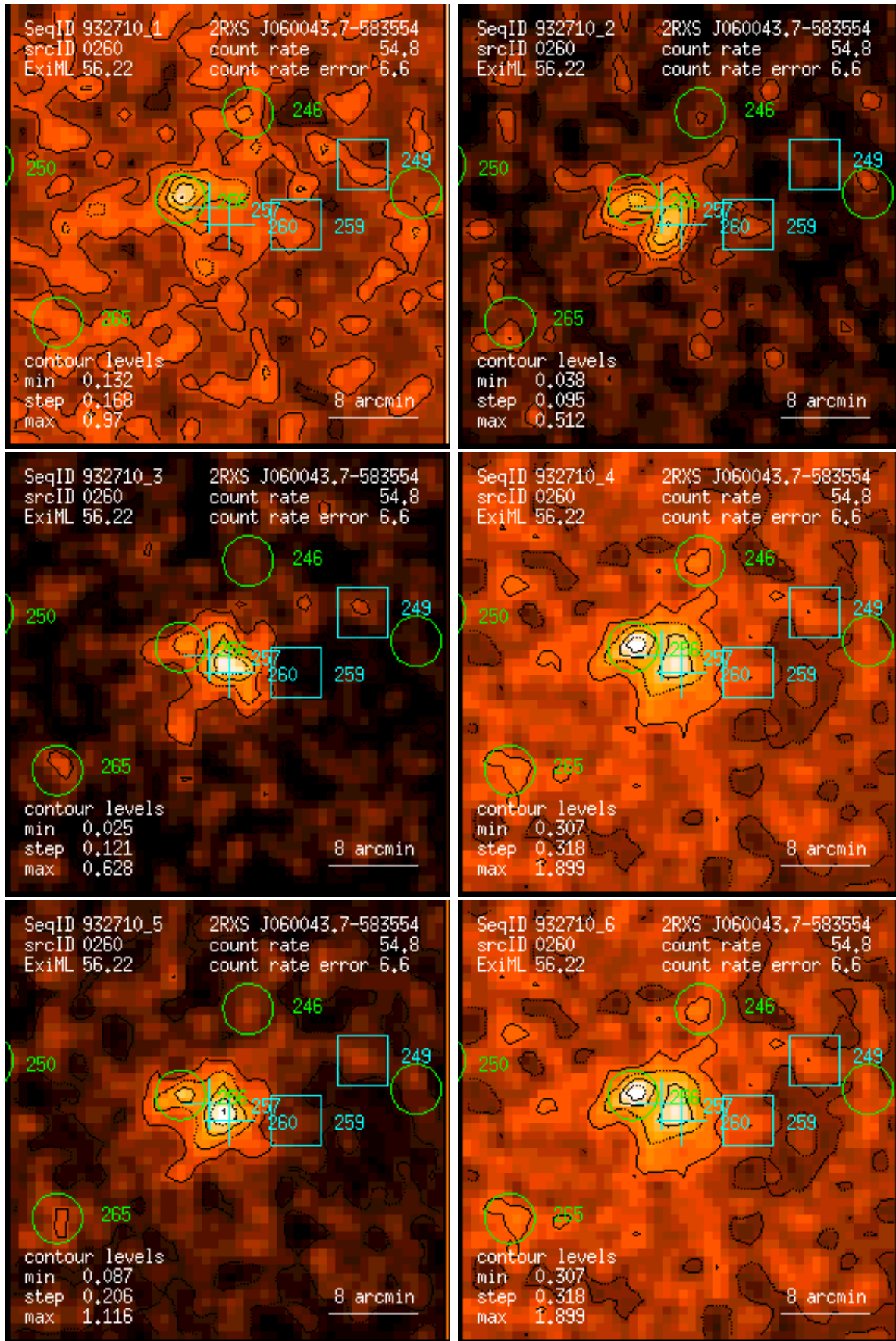
Figure 260: RASS 932710: detection 0260: band rate images, Gaussian filter: (1) PSPC channels 11 – 41, (2) 52 – 90, (3) 91 – 201, (4) 11 – 235, (5) 52 – 201, (6) 11 – 201. Broad band rates in counts/ks. Band rate contour levels in counts/ks/arcmin 2 .
