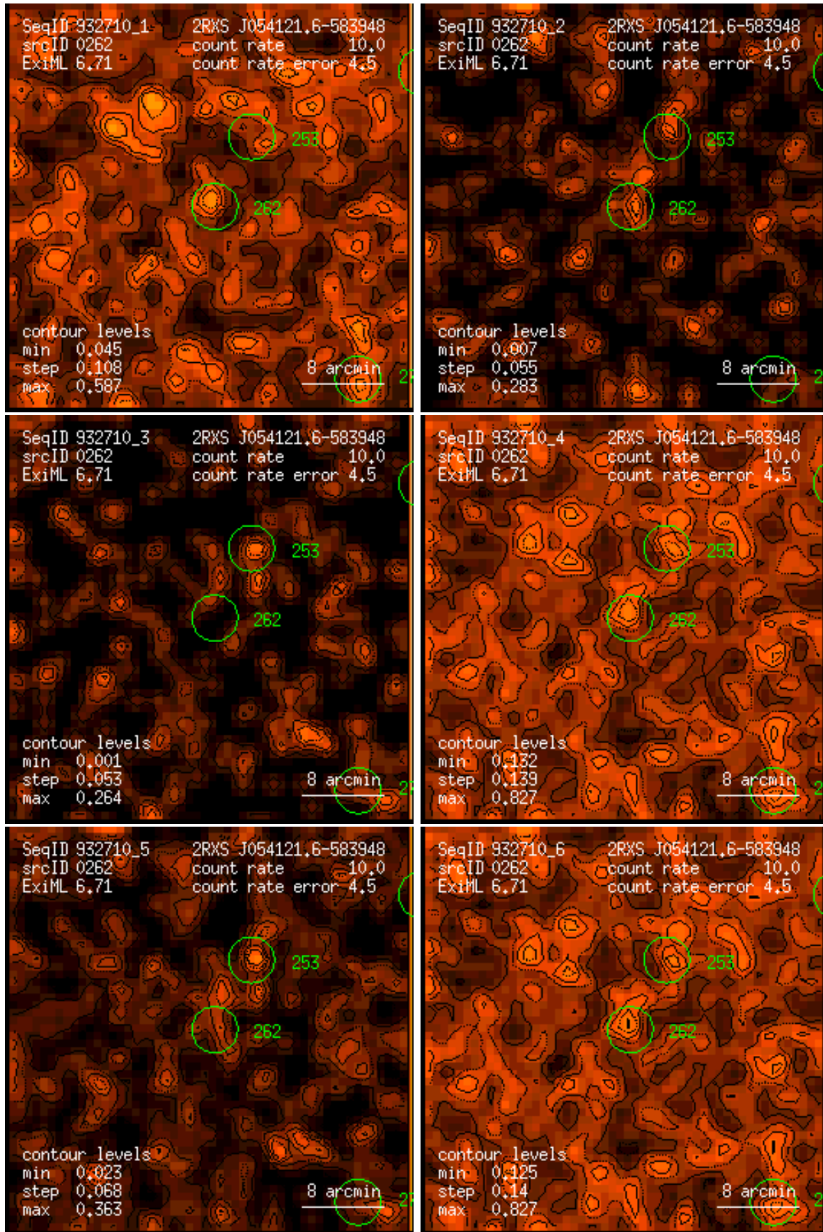
Figure 262: RASS 932710: detection 0262: band rate images, Gaussian filter: (1) PSPC channels 11 – 41, (2) 52 – 90, (3) 91 – 201, (4) 11 – 235, (5) 52 – 201, (6) 11 – 201. Broad band rates in counts/ks. Band rate contour levels in counts/ks/arcmin 2 .
