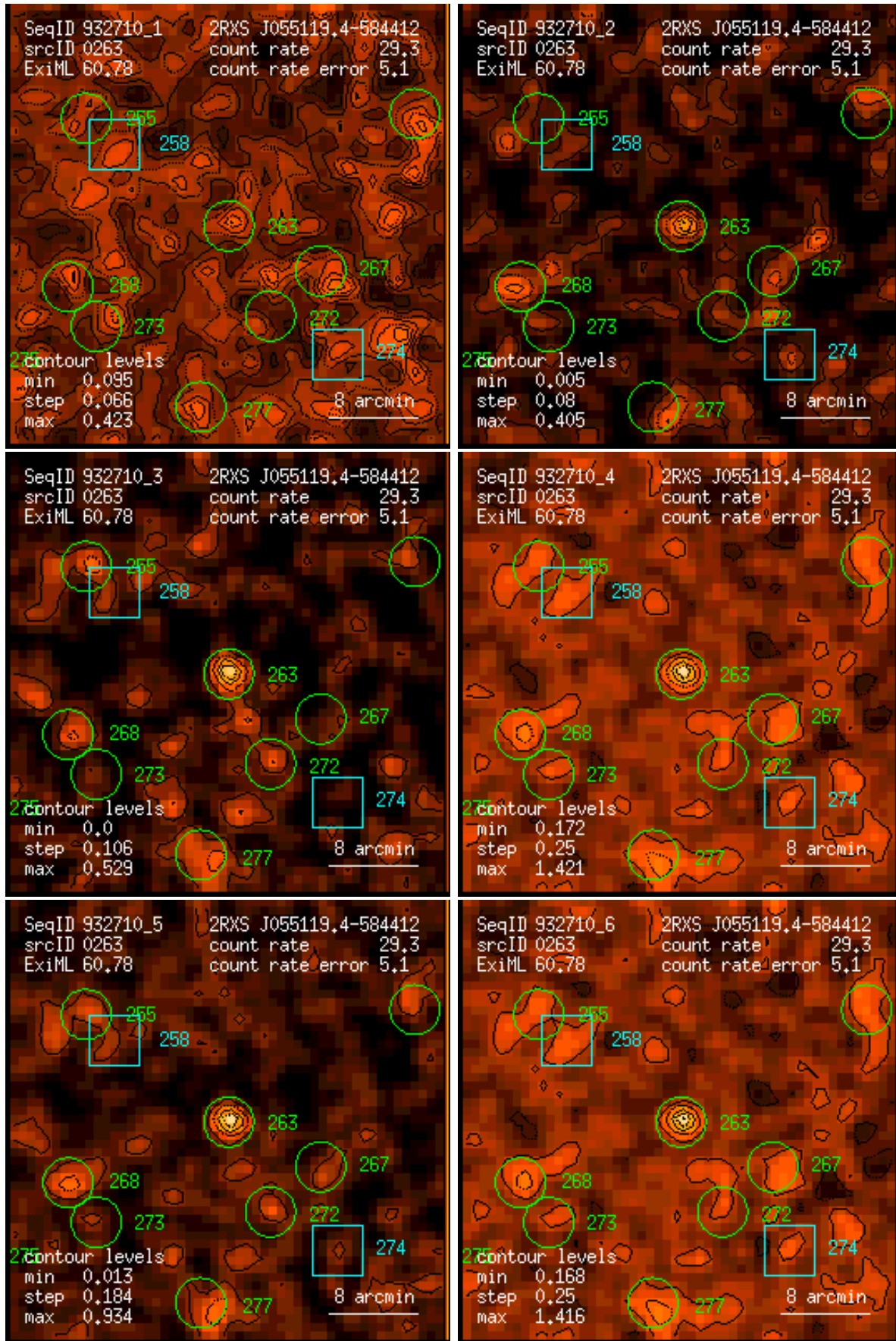
Figure 263: RASS 932710: detection 0263: band rate images, Gaussian filter: (1) PSPC channels 11 – 41, (2) 52 – 90, (3) 91 – 201, (4) 11 – 235, (5) 52 – 201, (6) 11 – 201. Broad band rates in counts/ks. Band rate contour levels in counts/ks/arcmin 2 .
