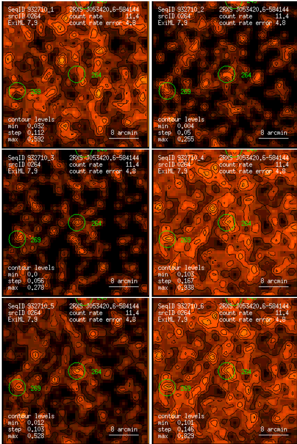
Figure 264: RASS 932710: detection 0264: band rate images, Gaussian filter: (1) PSPC channels 11 – 41, (2) 52 – 90, (3) 91 – 201, (4) 11 – 235, (5) 52 – 201, (6) 11 – 201. Broad band rates in counts/ks. Band rate contour levels in counts/ks/arcmin 2 .
