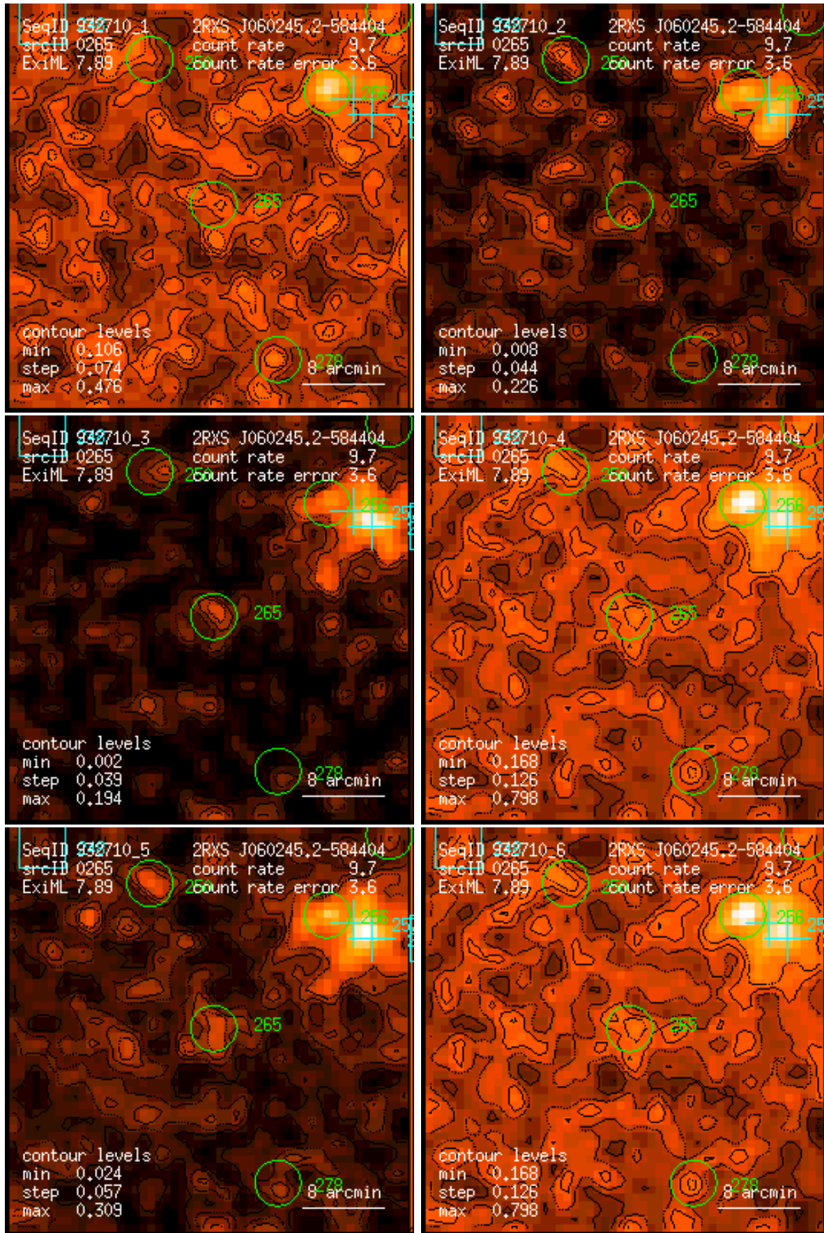
Figure 265: RASS 932710: detection 0265: band rate images, Gaussian filter: (1) PSPC channels 11 – 41, (2) 52 – 90, (3) 91 – 201, (4) 11 – 235, (5) 52 – 201, (6) 11 – 201. Broad band rates in counts/ks. Band rate contour levels in counts/ks/arcmin 2 .
