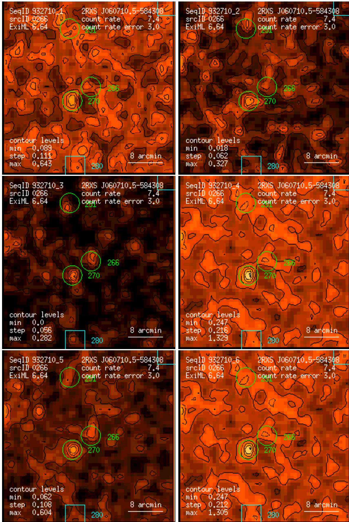
Figure 266: RASS 932710: detection 0266: band rate images, Gaussian filter: (1) PSPC channels 11 – 41, (2) 52 – 90, (3) 91 – 201, (4) 11 – 235, (5) 52 – 201, (6) 11 – 201. Broad band rates in counts/ks. Band rate contour levels in counts/ks/arcmin 2 .
