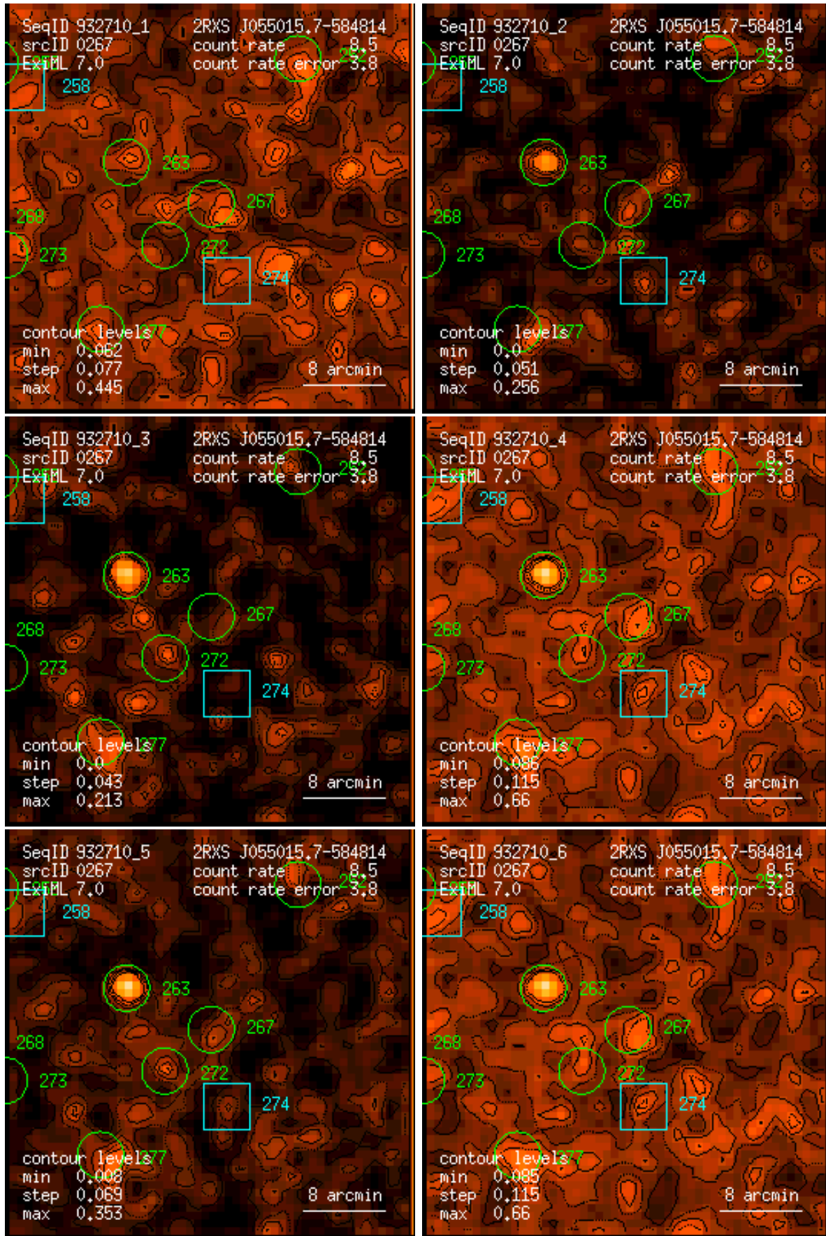
Figure 267: RASS 932710: detection 0267: band rate images, Gaussian filter: (1) PSPC channels 11 – 41, (2) 52 – 90, (3) 91 – 201, (4) 11 – 235, (5) 52 – 201, (6) 11 – 201. Broad band rates in counts/ks. Band rate contour levels in counts/ks/arcmin 2 .
