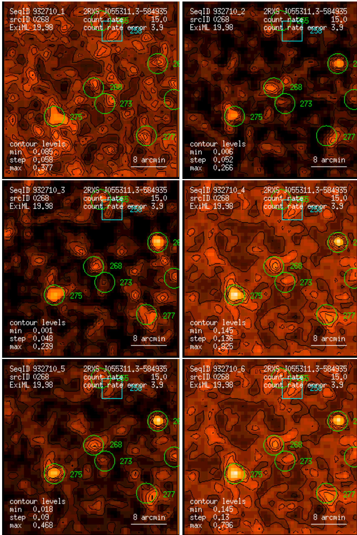
Figure 268: RASS 932710: detection 0268: band rate images, Gaussian filter: (1) PSPC channels 11 – 41, (2) 52 – 90, (3) 91 – 201, (4) 11 – 235, (5) 52 – 201, (6) 11 – 201. Broad band rates in counts/ks. Band rate contour levels in counts/ks/arcmin 2 .
