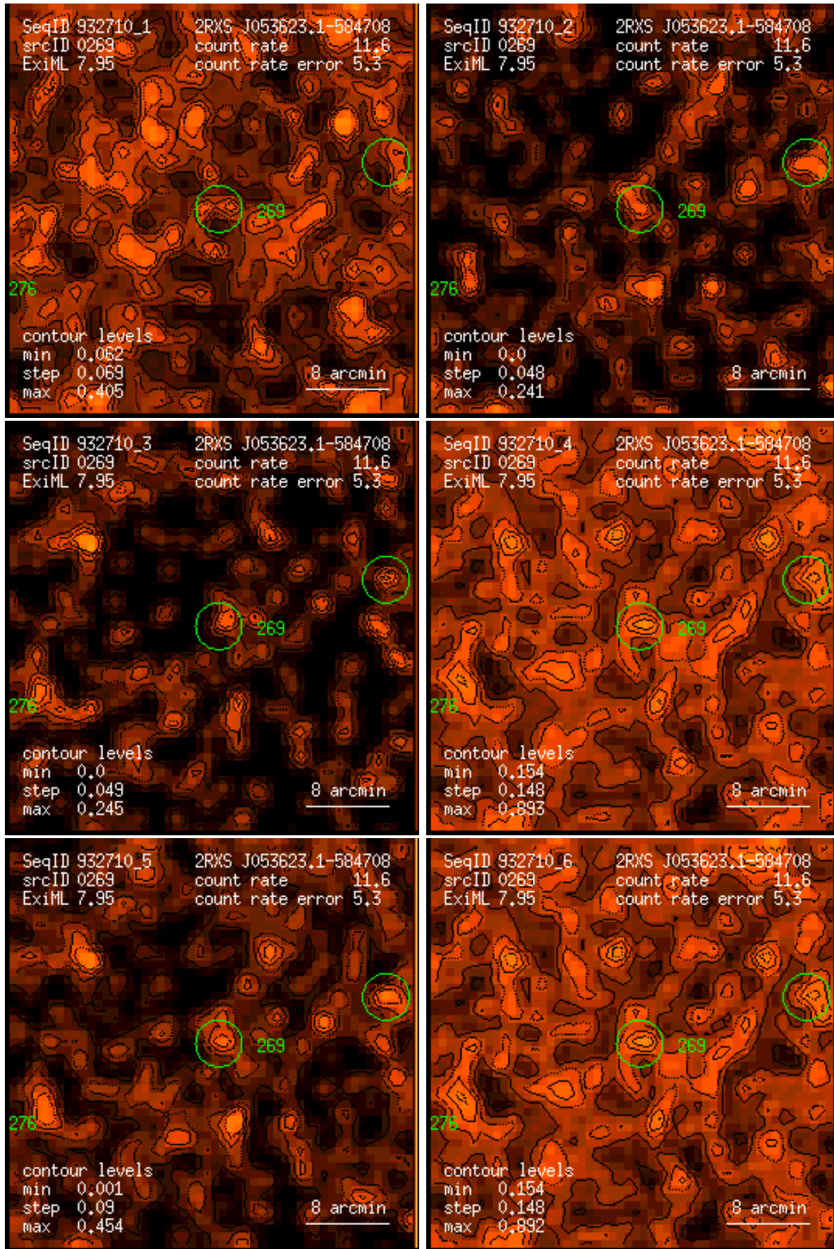
Figure 269: RASS 932710: detection 0269: band rate images, Gaussian filter: (1) PSPC channels 11 – 41, (2) 52 – 90, (3) 91 – 201, (4) 11 – 235, (5) 52 – 201, (6) 11 – 201. Broad band rates in counts/ks. Band rate contour levels in counts/ks/arcmin 2 .
