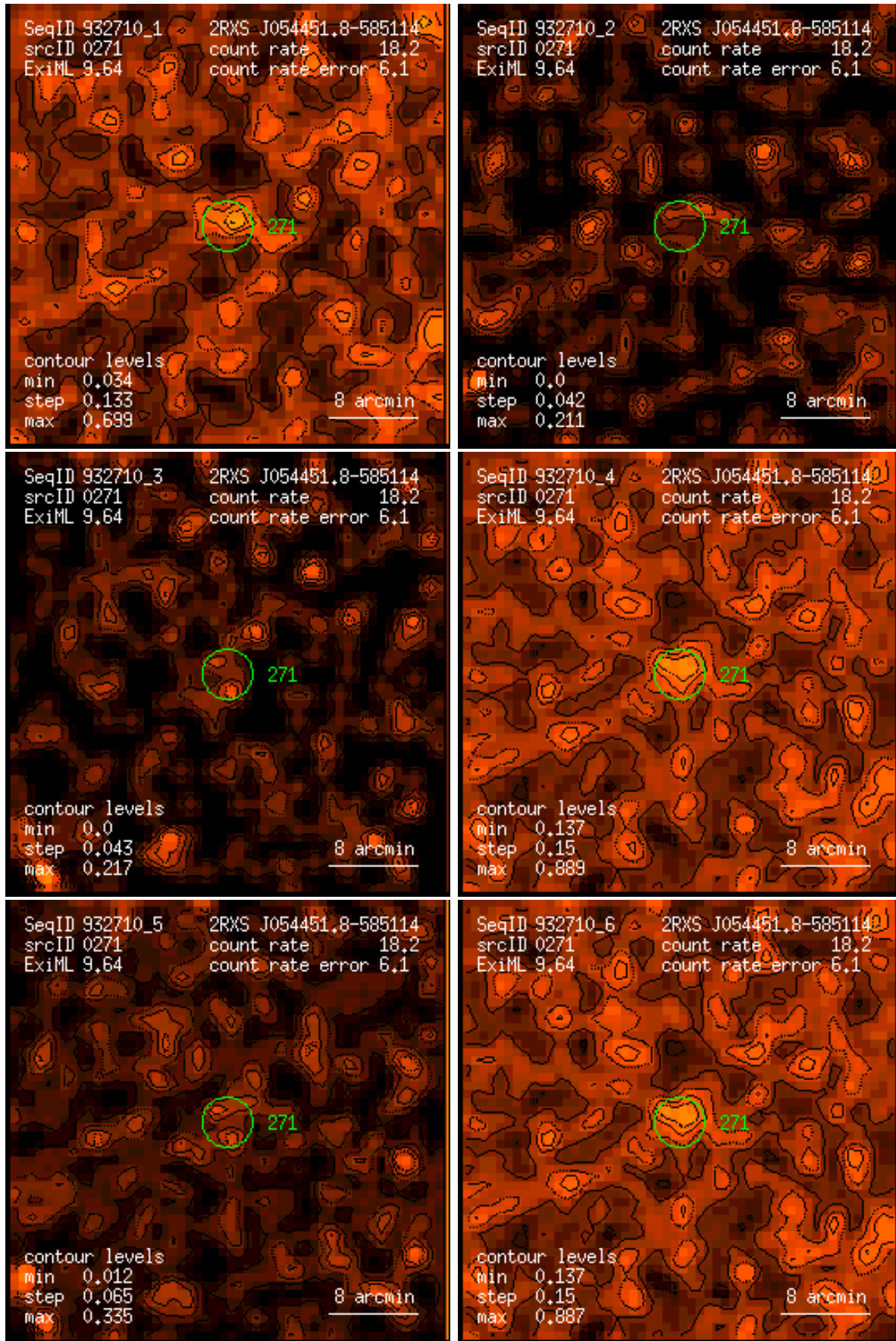
Figure 271: RASS 932710: detection 0271: band rate images, Gaussian filter: (1) PSPC channels 11 – 41, (2) 52 – 90, (3) 91 – 201, (4) 11 – 235, (5) 52 – 201, (6) 11 – 201. Broad band rates in counts/ks. Band rate contour levels in counts/ks/arcmin 2 .
