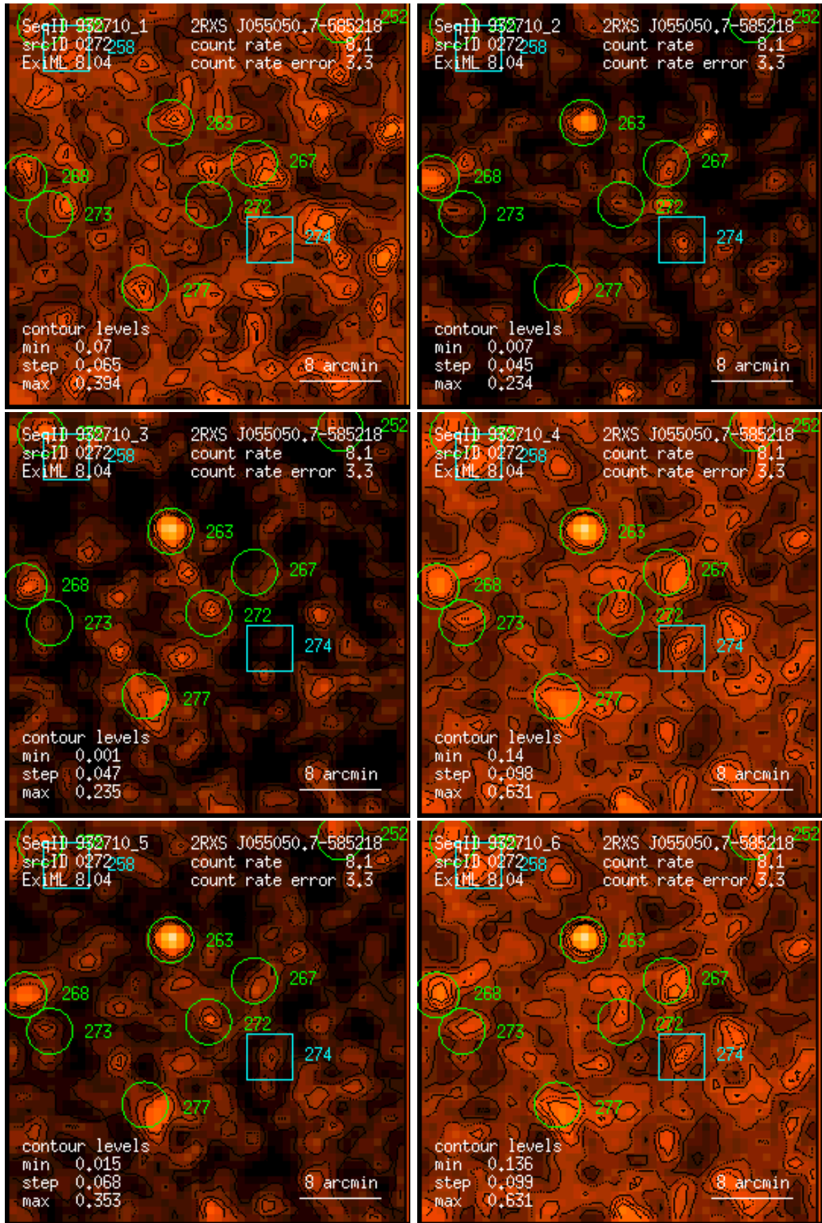
Figure 272: RASS 932710: detection 0272: band rate images, Gaussian filter: (1) PSPC channels 11 – 41, (2) 52 – 90, (3) 91 – 201, (4) 11 – 235, (5) 52 – 201, (6) 11 – 201. Broad band rates in counts/ks. Band rate contour levels in counts/ks/arcmin 2 .
