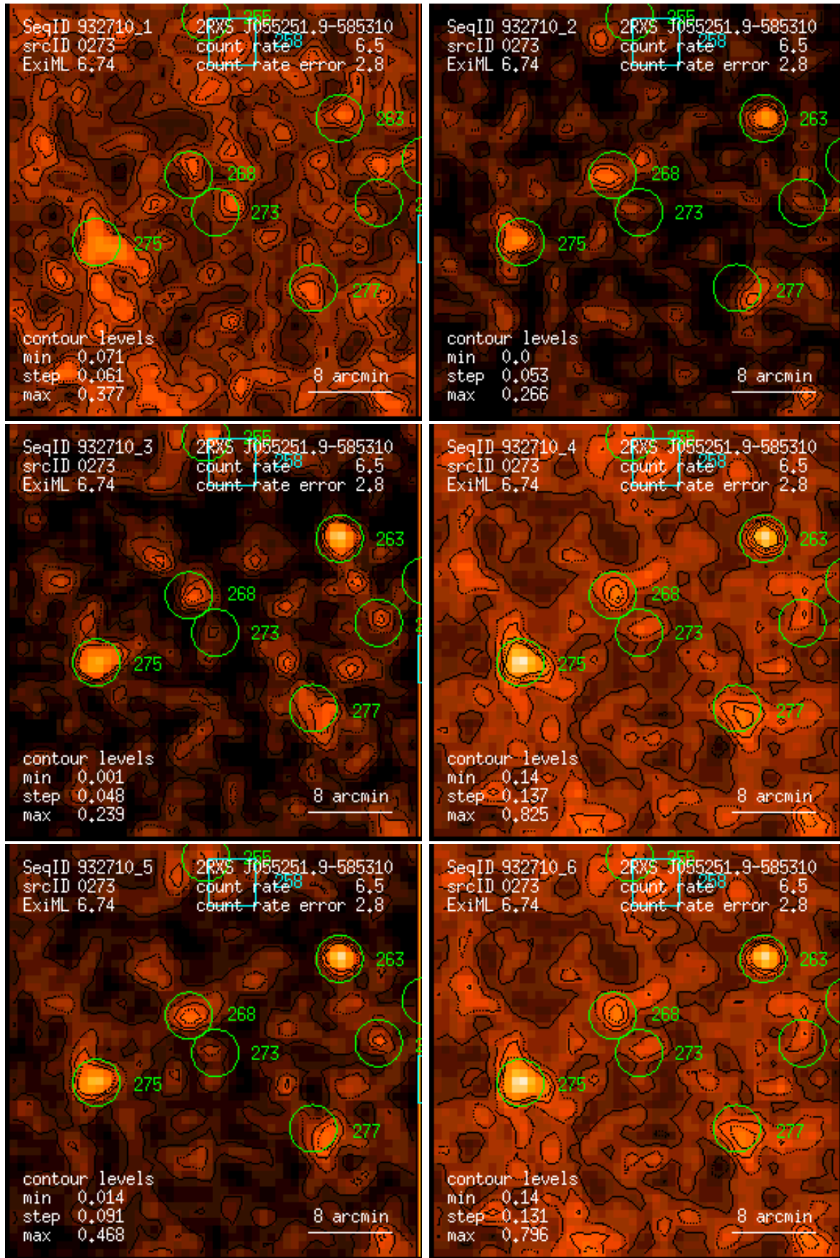
Figure 273: RASS 932710: detection 0273: band rate images, Gaussian filter: (1) PSPC channels 11 – 41, (2) 52 – 90, (3) 91 – 201, (4) 11 – 235, (5) 52 – 201, (6) 11 – 201. Broad band rates in counts/ks. Band rate contour levels in counts/ks/arcmin 2 .
