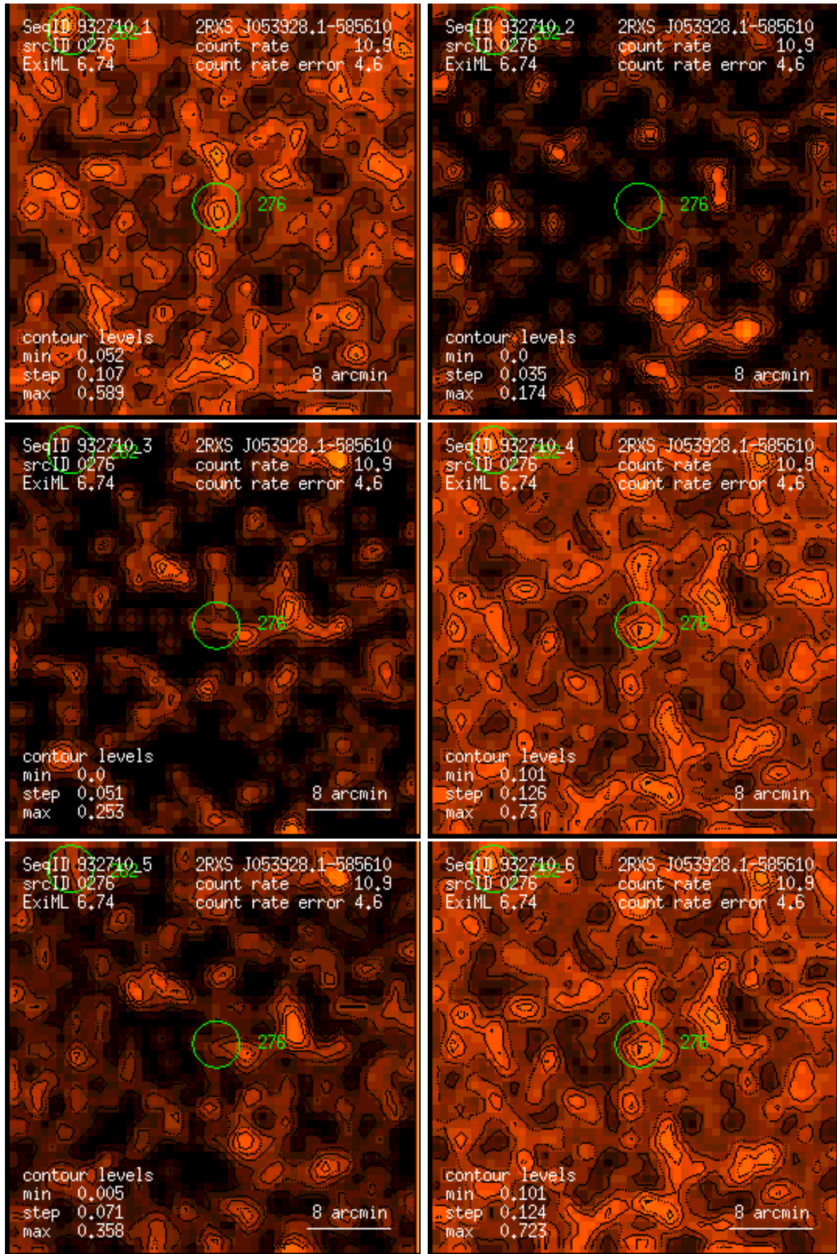
Figure 276: RASS 932710: detection 0276: band rate images, Gaussian filter: (1) PSPC channels 11 – 41, (2) 52 – 90, (3) 91 – 201, (4) 11 – 235, (5) 52 – 201, (6) 11 – 201. Broad band rates in counts/ks. Band rate contour levels in counts/ks/arcmin 2 .
