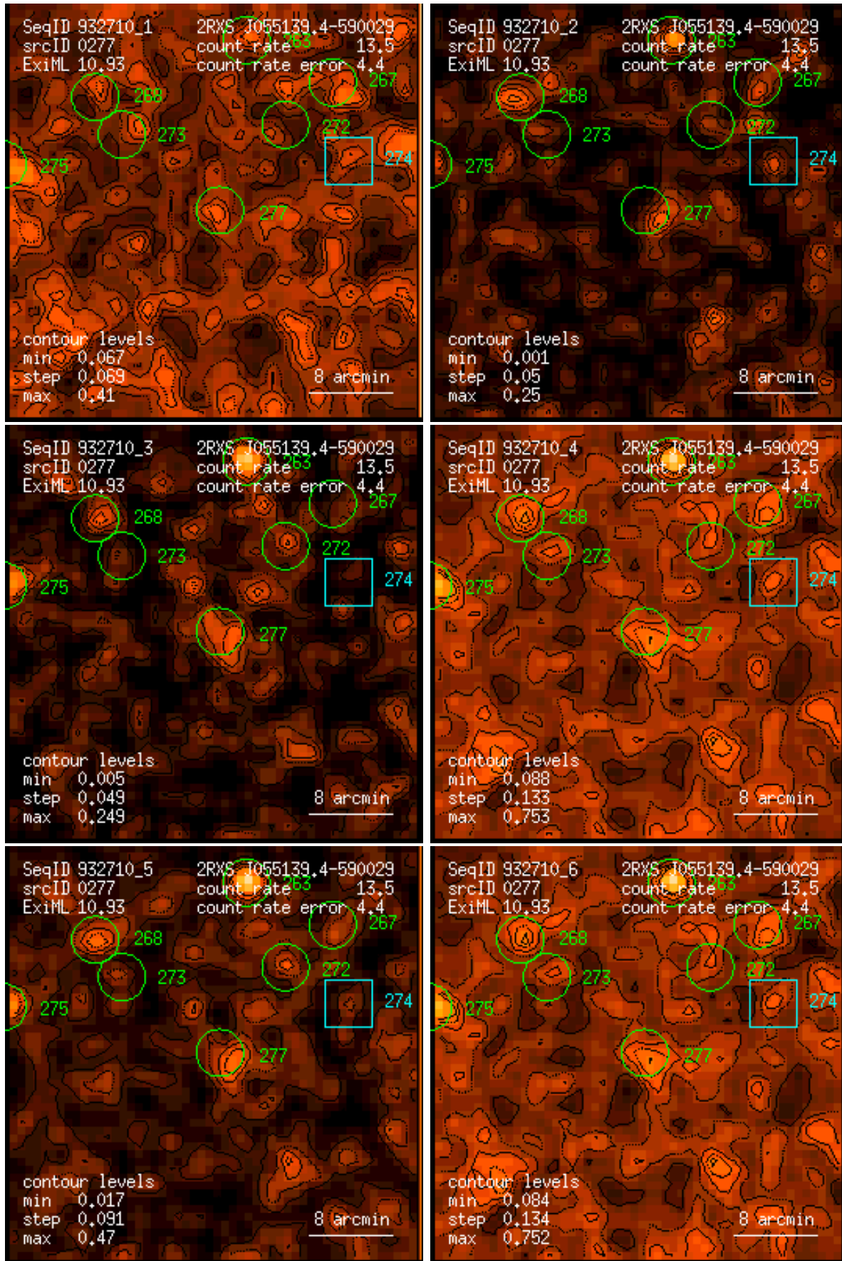
Figure 277: RASS 932710: detection 0277: band rate images, Gaussian filter: (1) PSPC channels 11 – 41, (2) 52 – 90, (3) 91 – 201, (4) 11 – 235, (5) 52 – 201, (6) 11 – 201. Broad band rates in counts/ks. Band rate contour levels in counts/ks/arcmin 2 .
