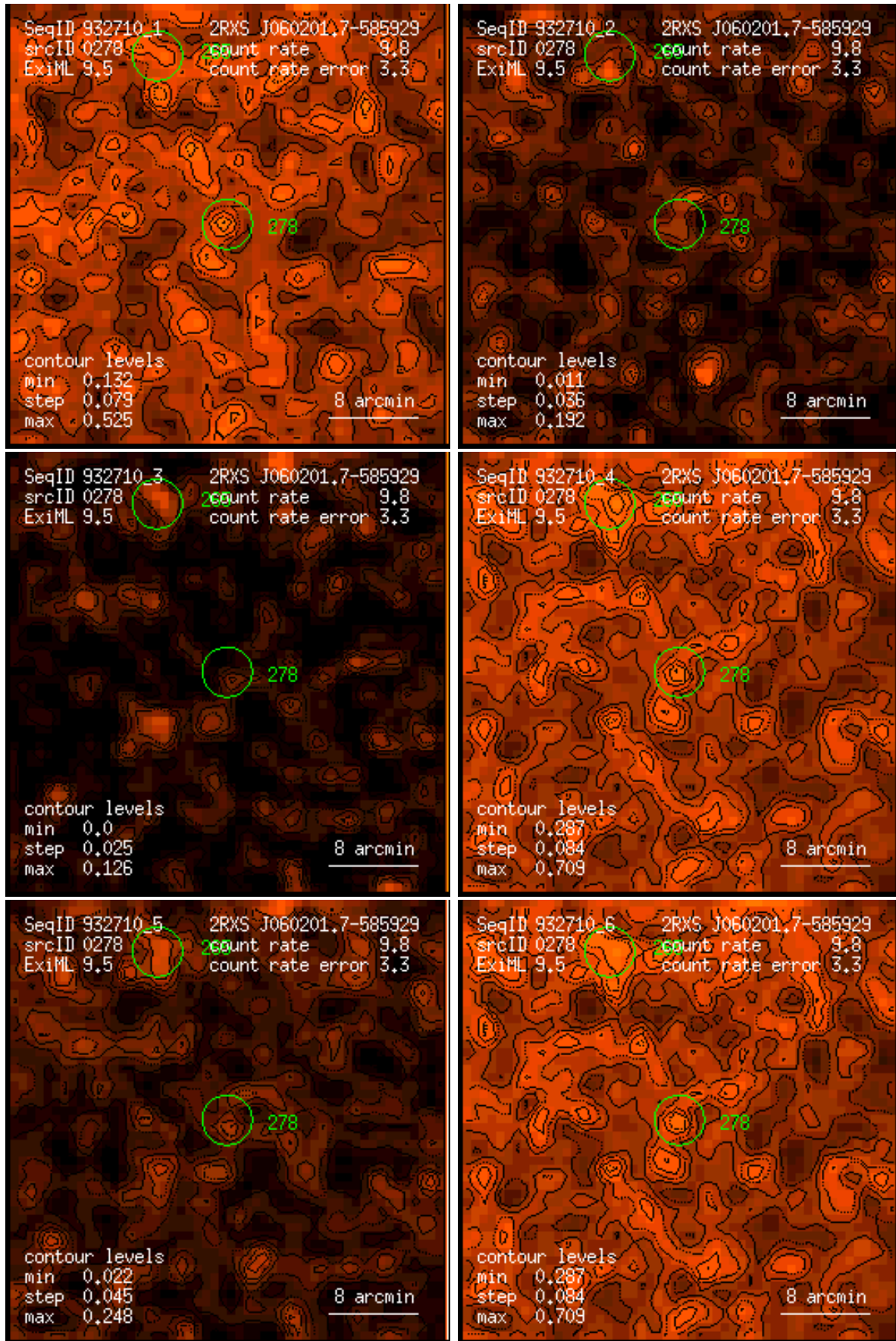
Figure 278: RASS 932710: detection 0278: band rate images, Gaussian filter: (1) PSPC channels 11 – 41, (2) 52 – 90, (3) 91 – 201, (4) 11 – 235, (5) 52 – 201, (6) 11 – 201. Broad band rates in counts/ks. Band rate contour levels in counts/ks/arcmin 2 .
