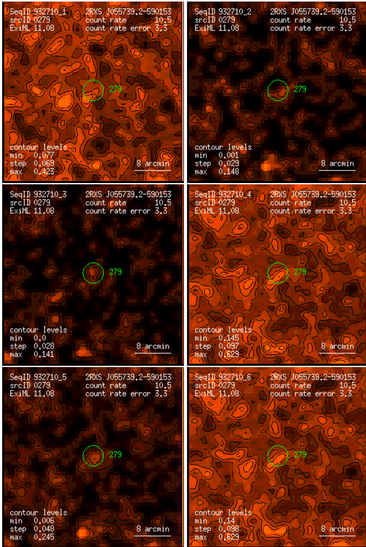
Figure 279: RASS 932710: detection 0279: band rate images, Gaussian filter: (1) PSPC channels 11 – 41, (2) 52 – 90, (3) 91 – 201, (4) 11 – 235, (5) 52 – 201, (6) 11 – 201. Broad band rates in counts/ks. Band rate contour levels in counts/ks/arcmin 2 .
