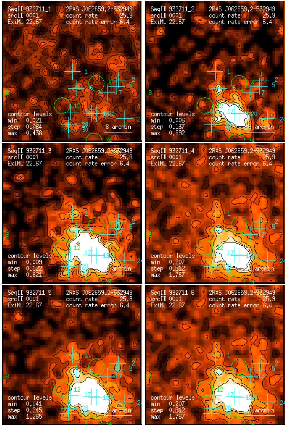
Figure 1: RASS 932711: detection 0001: band rate images, Gaussian filter: (1) PSPC channels 11 – 41, (2) 52 – 90, (3) 91 – 201, (4) 11 – 235, (5) 52 – 201, (6) 11 – 201. Broad band rates in counts/ks. Band rate contour levels in counts/ks/arcmin 2 .
