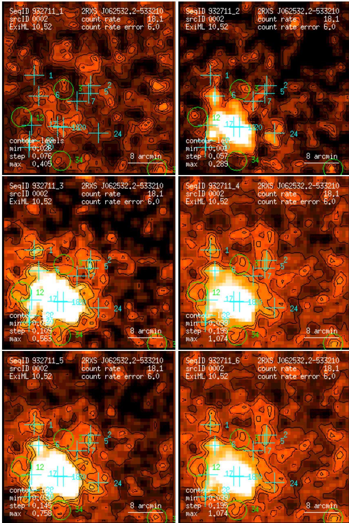
Figure 2: RASS 932711: detection 0002: band rate images, Gaussian filter: (1) PSPC channels 11 – 41, (2) 52 – 90, (3) 91 – 201, (4) 11 – 235, (5) 52 – 201, (6) 11 – 201. Broad band rates in counts/ks. Band rate contour levels in counts/ks/arcmin 2 .
