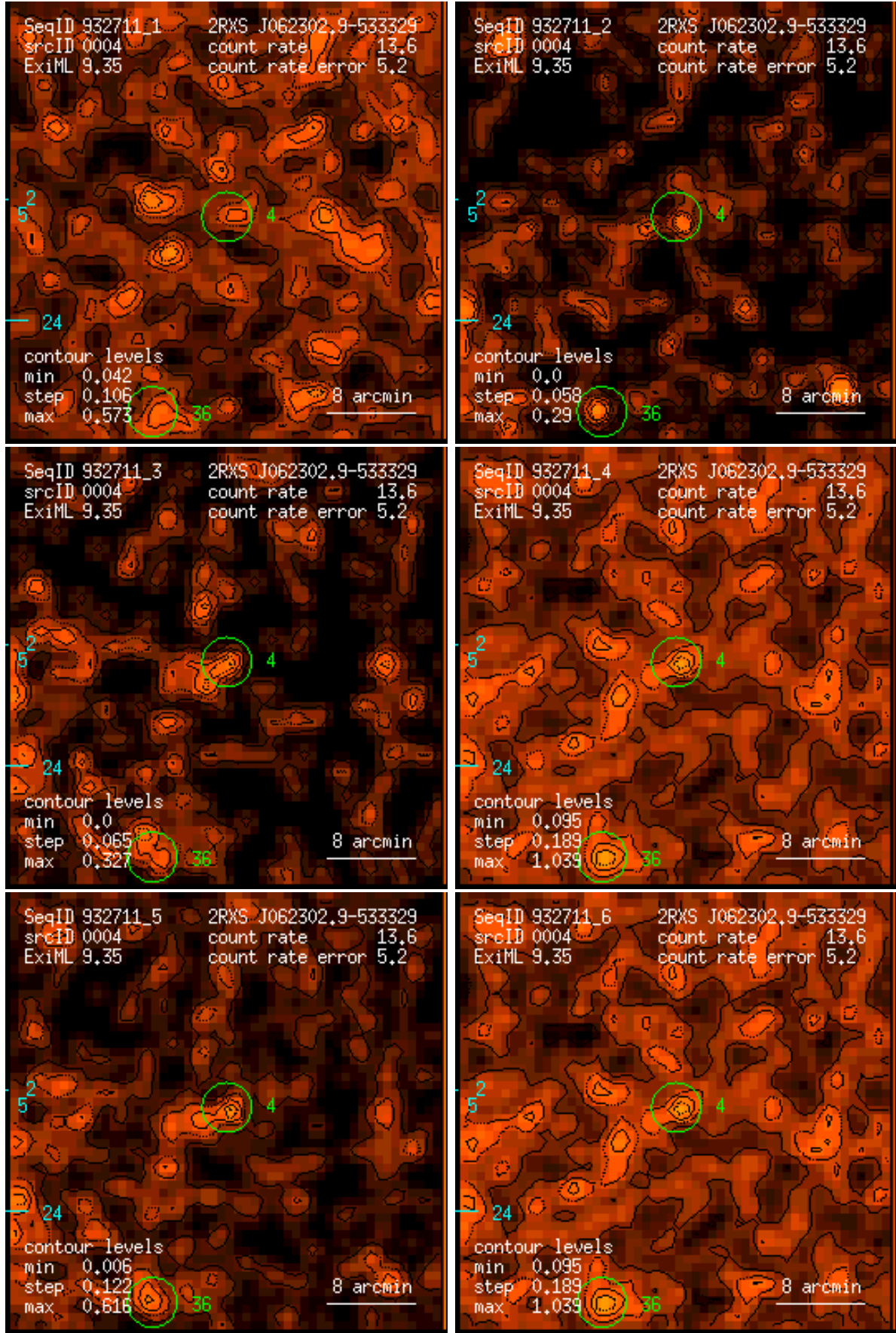
Figure 4: RASS 932711: detection 0004: band rate images, Gaussian filter: (1) PSPC channels 11 – 41, (2) 52 – 90, (3) 91 – 201, (4) 11 – 235, (5) 52 – 201, (6) 11 – 201. Broad band rates in counts/ks. Band rate contour levels in counts/ks/arcmin 2 .
