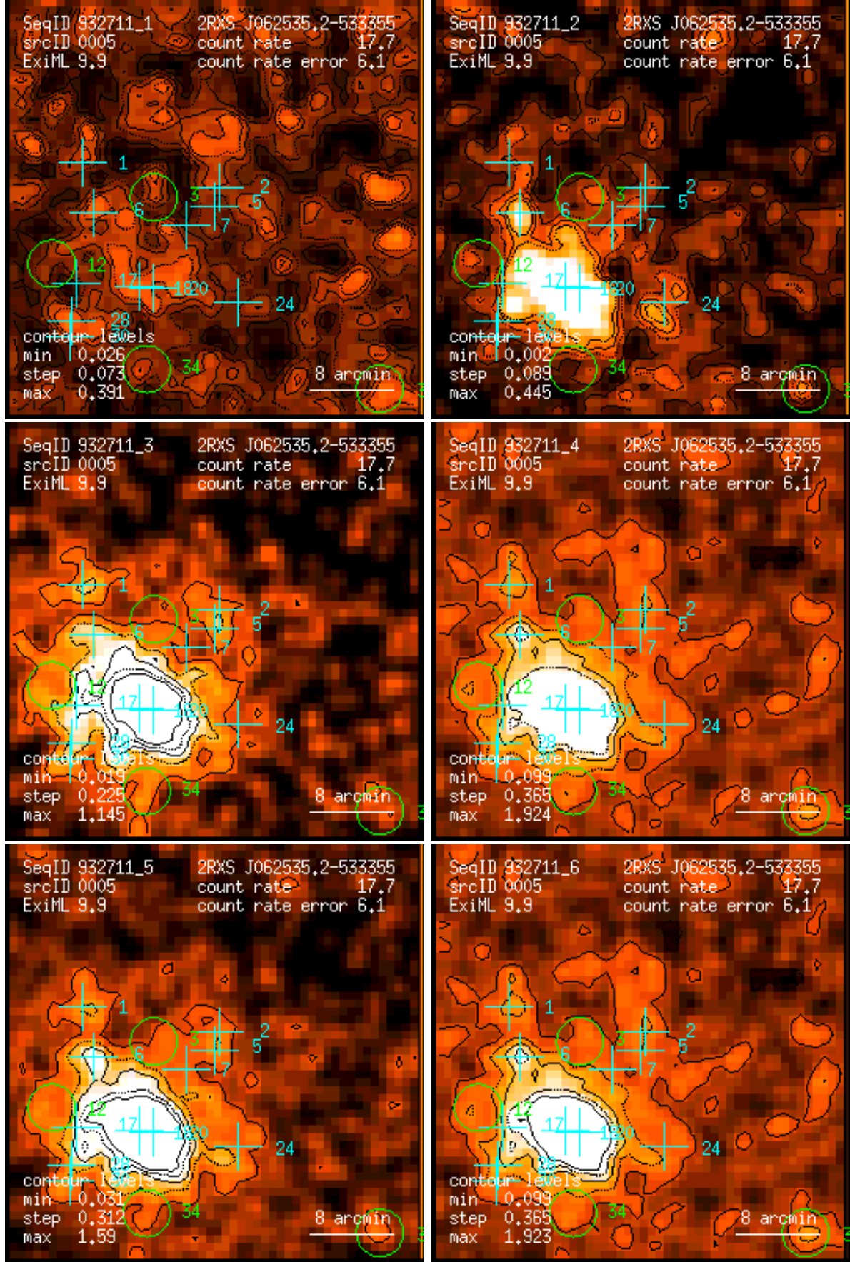
Figure 5: RASS 932711: detection 0005: band rate images, Gaussian filter: (1) PSPC channels 11 – 41, (2) 52 – 90, (3) 91 – 201, (4) 11 – 235, (5) 52 – 201, (6) 11 – 201. Broad band rates in counts/ks. Band rate contour levels in counts/ks/arcmin 2 .
