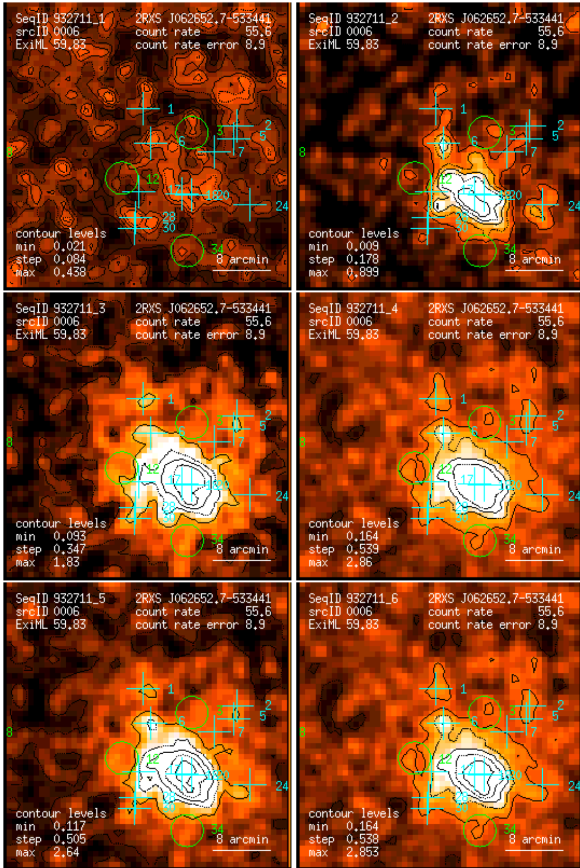
Figure 6: RASS 932711: detection 0006: band rate images, Gaussian filter: (1) PSPC channels 11 – 41, (2) 52 – 90, (3) 91 – 201, (4) 11 – 235, (5) 52 – 201, (6) 11 – 201. Broad band rates in counts/ks. Band rate contour levels in counts/ks/arcmin 2 .
