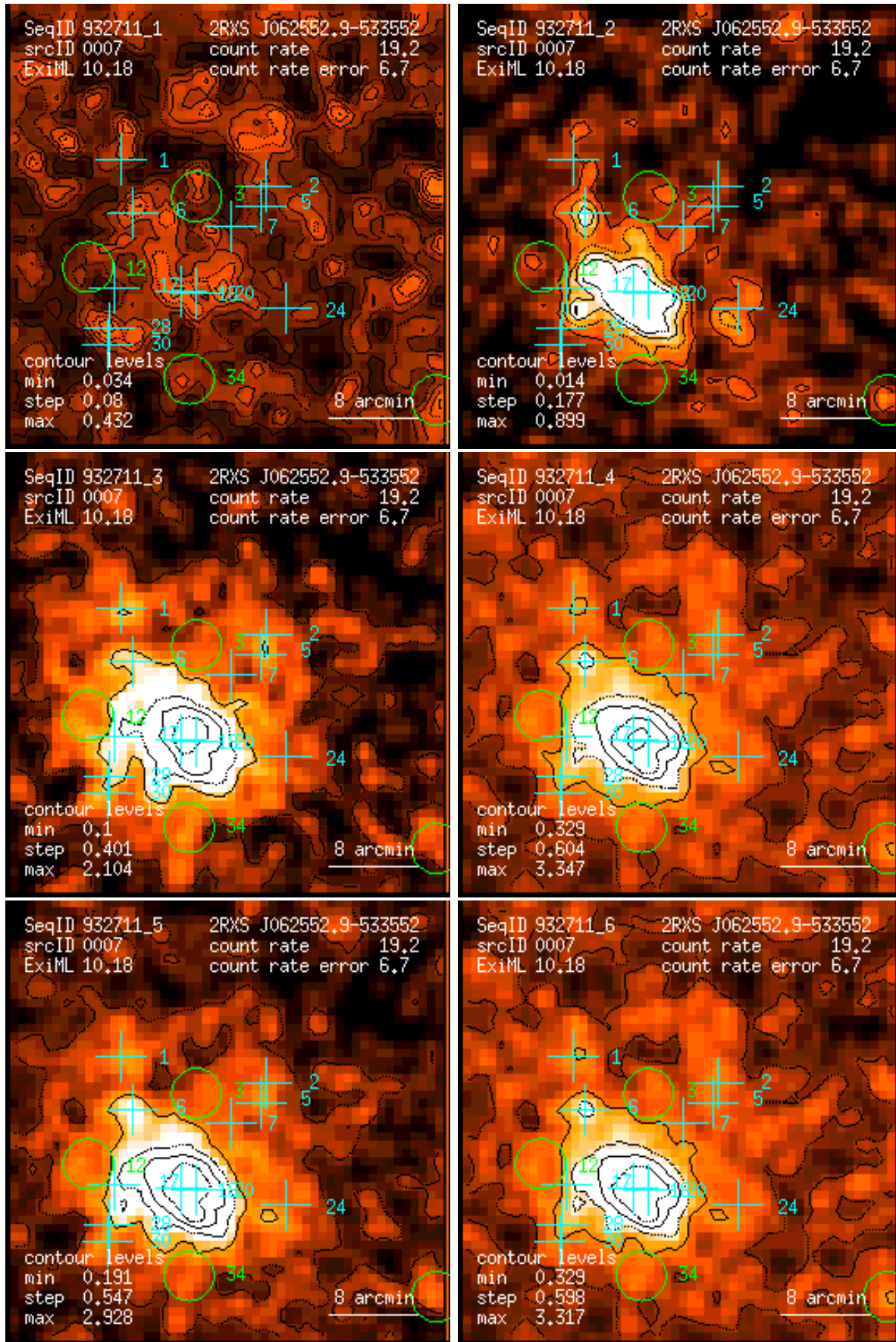
Figure 7: RASS 932711: detection 0007: band rate images, Gaussian filter: (1) PSPC channels 11 – 41, (2) 52 – 90, (3) 91 – 201, (4) 11 – 235, (5) 52 – 201, (6) 11 – 201. Broad band rates in counts/ks. Band rate contour levels in counts/ks/arcmin 2 .
