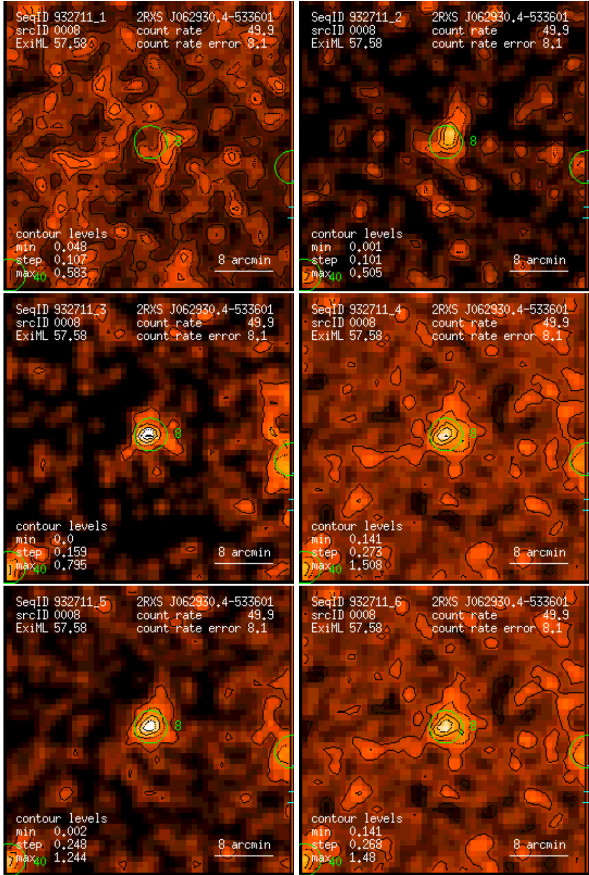
Figure 8: RASS 932711: detection 0008: band rate images, Gaussian filter: (1) PSPC channels 11 – 41, (2) 52 – 90, (3) 91 – 201, (4) 11 – 235, (5) 52 – 201, (6) 11 – 201. Broad band rates in counts/ks. Band rate contour levels in counts/ks/arcmin 2 .
