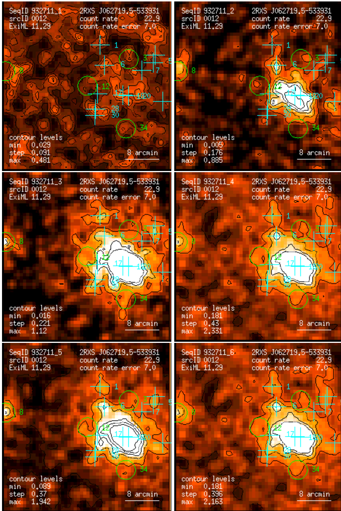
Figure 12: RASS 932711: detection 0012: band rate images, Gaussian filter: (1) PSPC channels 11 – 41, (2) 52 – 90, (3) 91 – 201, (4) 11 – 235, (5) 52 – 201, (6) 11 – 201. Broad band rates in counts/ks. Band rate contour levels in counts/ks/arcmin 2 .
