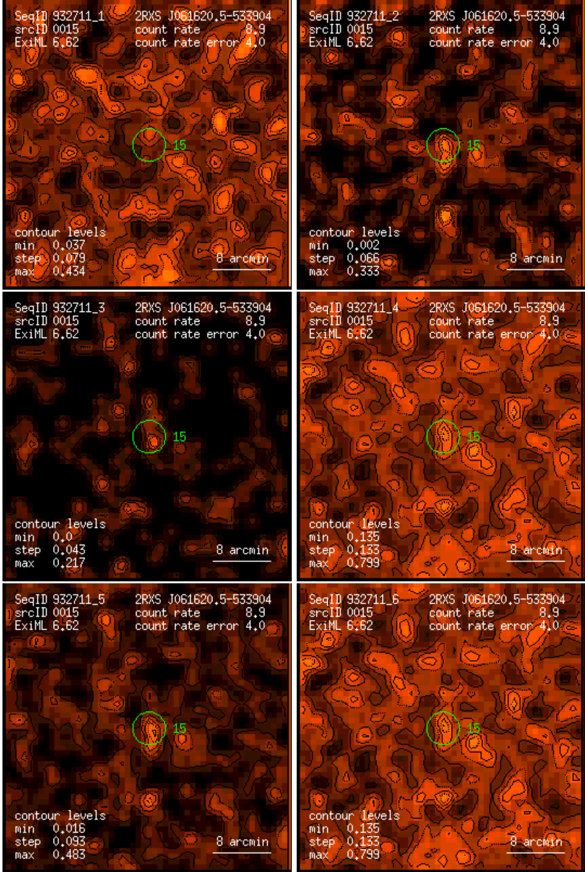
Figure 15: RASS 932711: detection 0015: band rate images, Gaussian filter: (1) PSPC channels 11 – 41, (2) 52 – 90, (3) 91 – 201, (4) 11 – 235, (5) 52 – 201, (6) 11 – 201. Broad band rates in counts/ks. Band rate contour levels in counts/ks/arcmin 2 .
