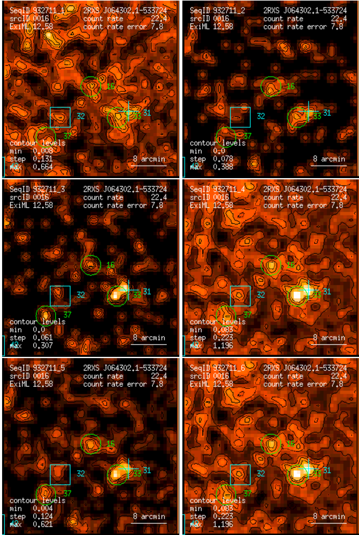
Figure 16: RASS 932711: detection 0016: band rate images, Gaussian filter: (1) PSPC channels 11 – 41, (2) 52 – 90, (3) 91 – 201, (4) 11 – 235, (5) 52 – 201, (6) 11 – 201. Broad band rates in counts/ks. Band rate contour levels in counts/ks/arcmin 2 .
