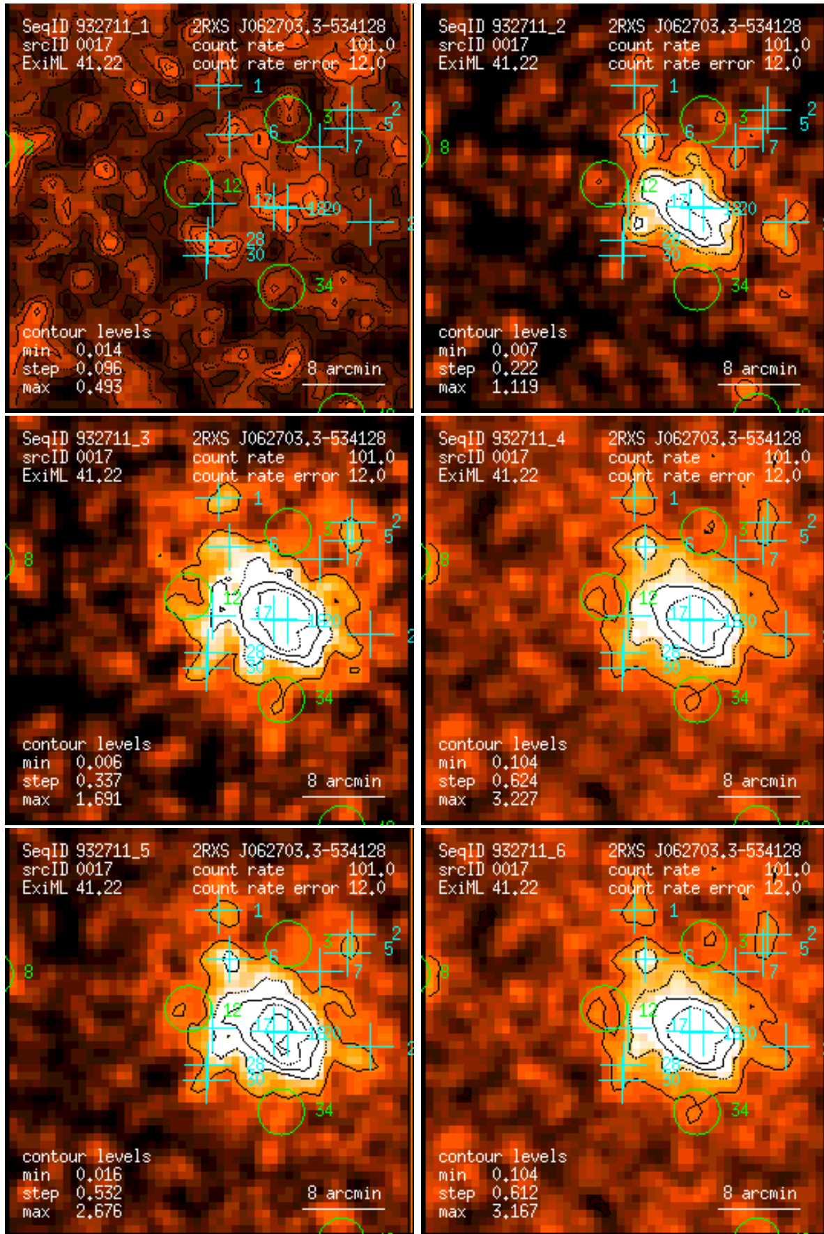
Figure 17: RASS 932711: detection 0017: band rate images, Gaussian filter: (1) PSPC channels 11 – 41, (2) 52 – 90, (3) 91 – 201, (4) 11 – 235, (5) 52 – 201, (6) 11 – 201. Broad band rates in counts/ks. Band rate contour levels in counts/ks/arcmin 2 .
