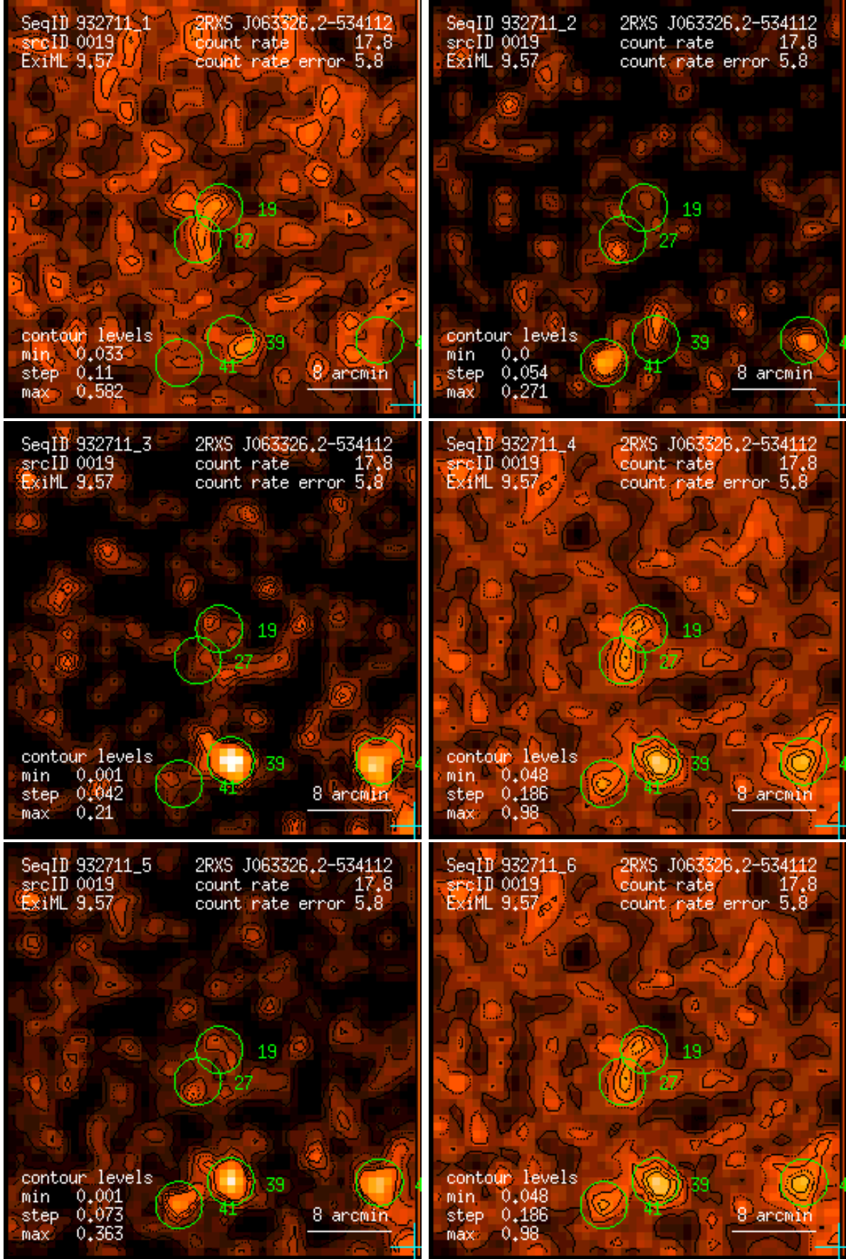
Figure 19: RASS 932711: detection 0019: band rate images, Gaussian filter: (1) PSPC channels 11 – 41, (2) 52 – 90, (3) 91 – 201, (4) 11 – 235, (5) 52 – 201, (6) 11 – 201. Broad band rates in counts/ks. Band rate contour levels in counts/ks/arcmin 2 .
