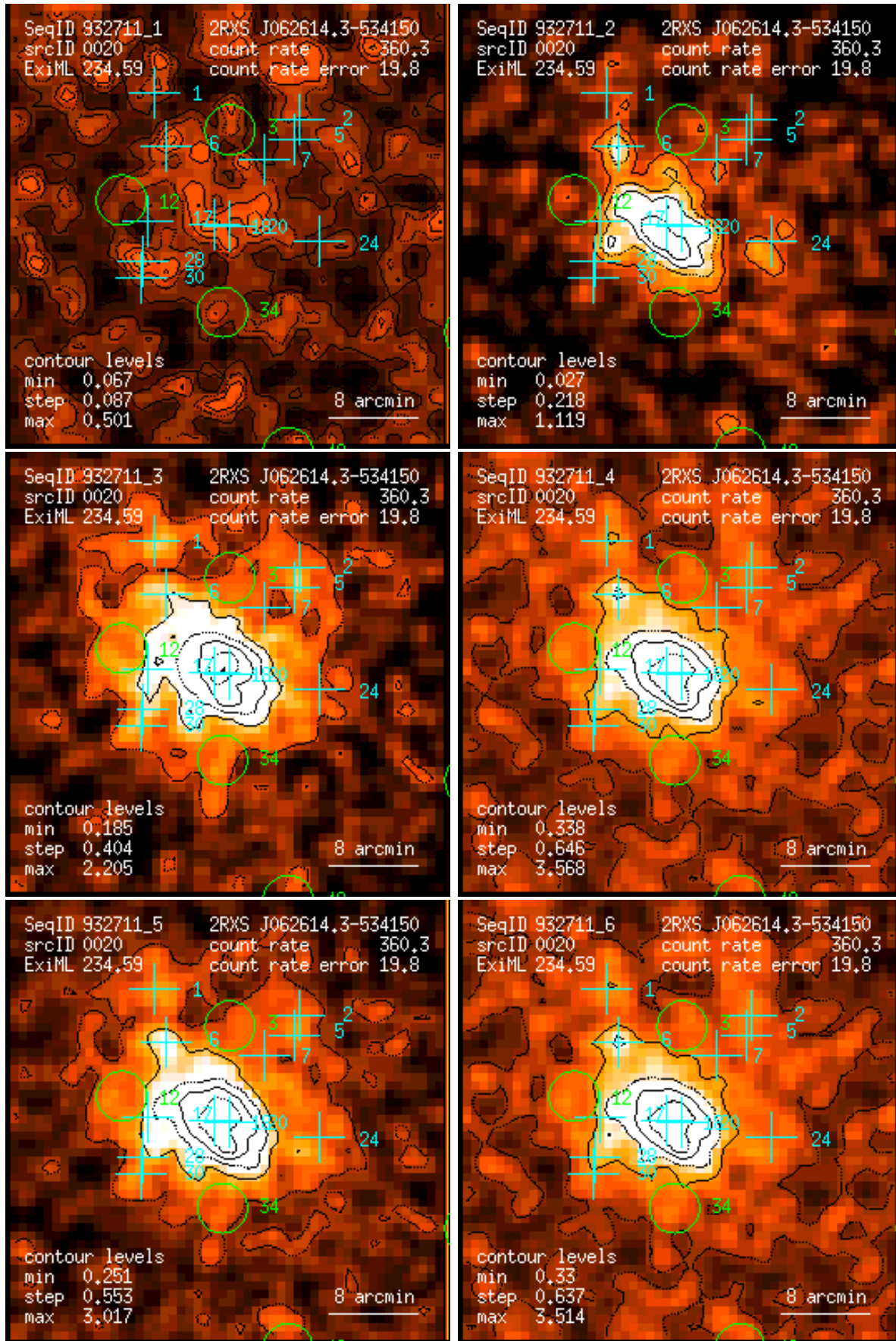
Figure 20: RASS 932711: detection 0020: band rate images, Gaussian filter: (1) PSPC channels 11 – 41, (2) 52 – 90, (3) 91 – 201, (4) 11 – 235, (5) 52 – 201, (6) 11 – 201. Broad band rates in counts/ks. Band rate contour levels in counts/ks/arcmin 2 .
