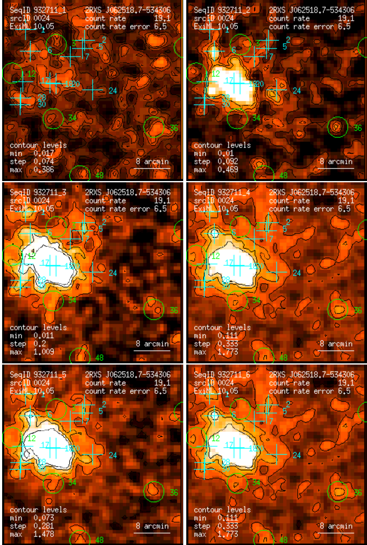
Figure 24: RASS 932711: detection 0024: band rate images, Gaussian filter: (1) PSPC channels 11 – 41, (2) 52 – 90, (3) 91 – 201, (4) 11 – 235, (5) 52 – 201, (6) 11 – 201. Broad band rates in counts/ks. Band rate contour levels in counts/ks/arcmin 2 .
