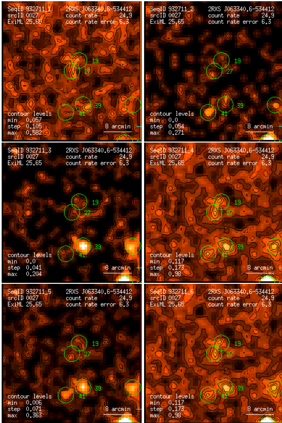
Figure 27: RASS 932711: detection 0027: band rate images, Gaussian filter: (1) PSPC channels 11 – 41, (2) 52 – 90, (3) 91 – 201, (4) 11 – 235, (5) 52 – 201, (6) 11 – 201. Broad band rates in counts/ks. Band rate contour levels in counts/ks/arcmin 2 .
