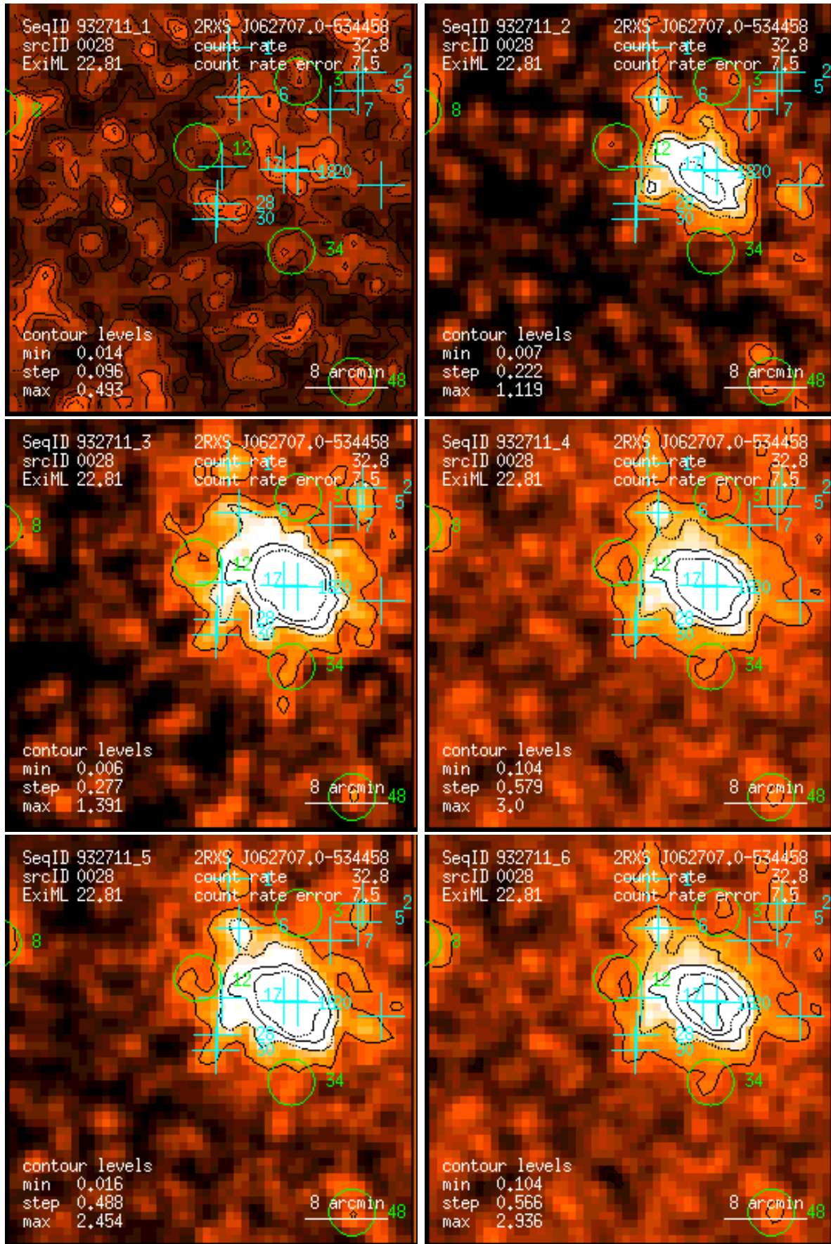
Figure 28: RASS 932711: detection 0028: band rate images, Gaussian filter: (1) PSPC channels 11 – 41, (2) 52 – 90, (3) 91 – 201, (4) 11 – 235, (5) 52 – 201, (6) 11 – 201. Broad band rates in counts/ks. Band rate contour levels in counts/ks/arcmin 2 .
