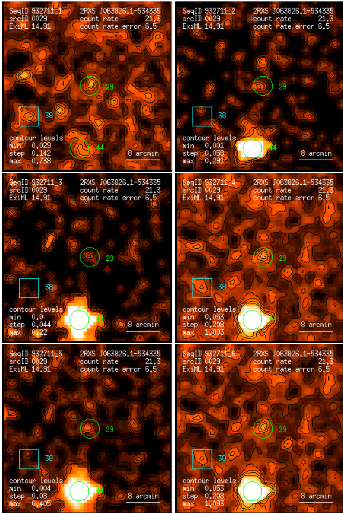
Figure 29: RASS 932711: detection 0029: band rate images, Gaussian filter: (1) PSPC channels 11 – 41, (2) 52 – 90, (3) 91 – 201, (4) 11 – 235, (5) 52 – 201, (6) 11 – 201. Broad band rates in counts/ks. Band rate contour levels in counts/ks/arcmin 2 .
