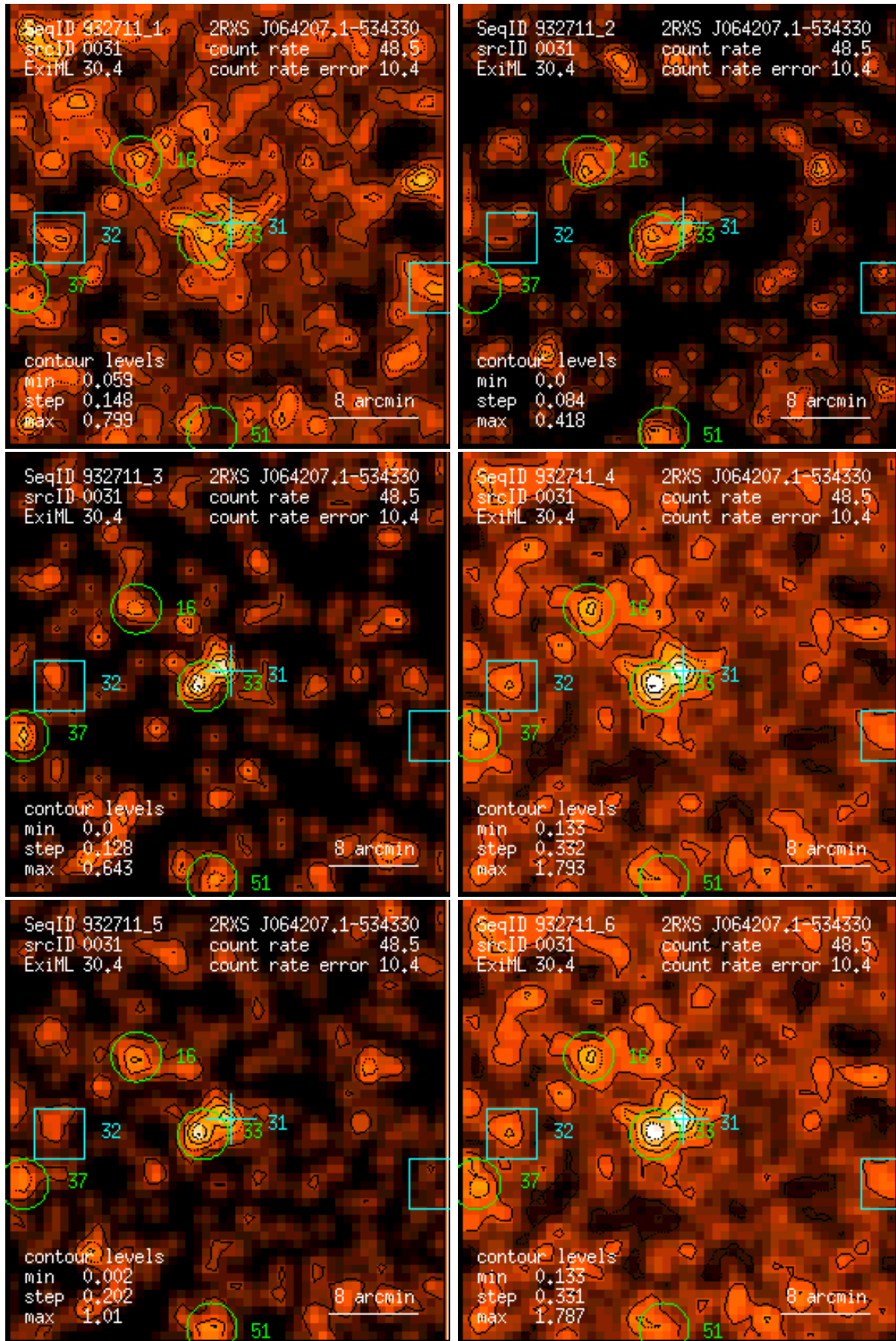
Figure 31: RASS 932711: detection 0031: band rate images, Gaussian filter: (1) PSPC channels 11 – 41, (2) 52 – 90, (3) 91 – 201, (4) 11 – 235, (5) 52 – 201, (6) 11 – 201. Broad band rates in counts/ks. Band rate contour levels in counts/ks/arcmin 2 .
