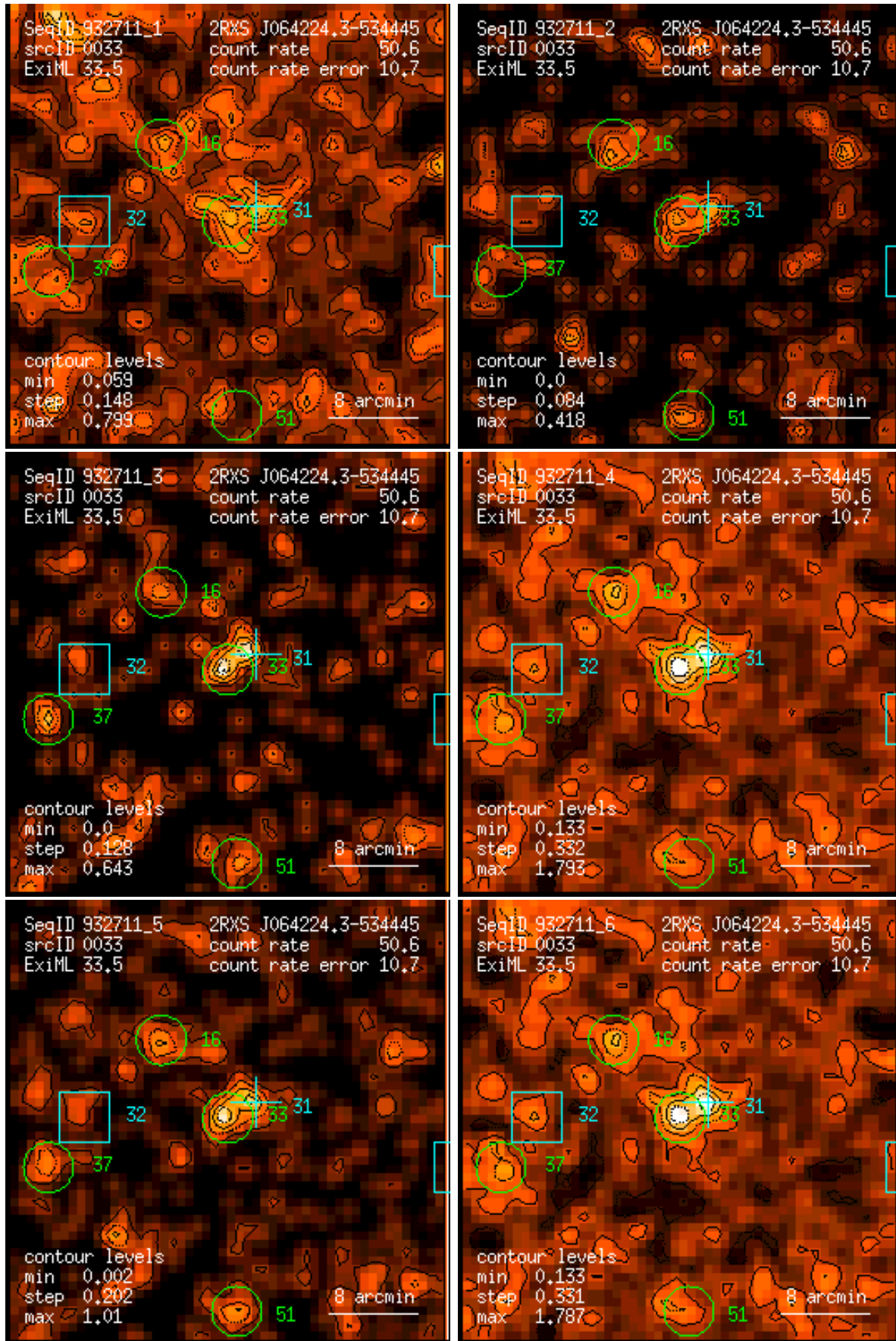
Figure 33: RASS 932711: detection 0033: band rate images, Gaussian filter: (1) PSPC channels 11 – 41, (2) 52 – 90, (3) 91 – 201, (4) 11 – 235, (5) 52 – 201, (6) 11 – 201. Broad band rates in counts/ks. Band rate contour levels in counts/ks/arcmin 2 .
