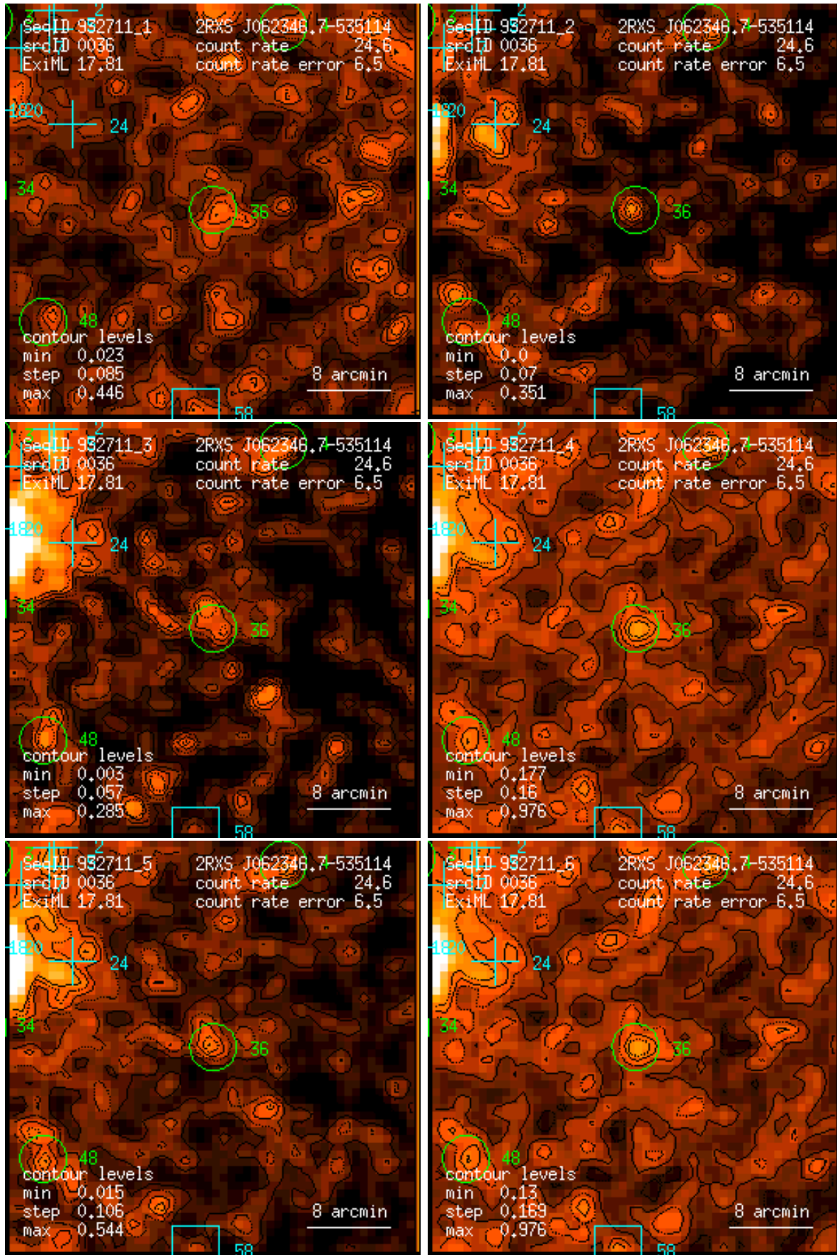
Figure 36: RASS 932711: detection 0036: band rate images, Gaussian filter: (1) PSPC channels 11 – 41, (2) 52 – 90, (3) 91 – 201, (4) 11 – 235, (5) 52 – 201, (6) 11 – 201. Broad band rates in counts/ks. Band rate contour levels in counts/ks/arcmin 2 .
