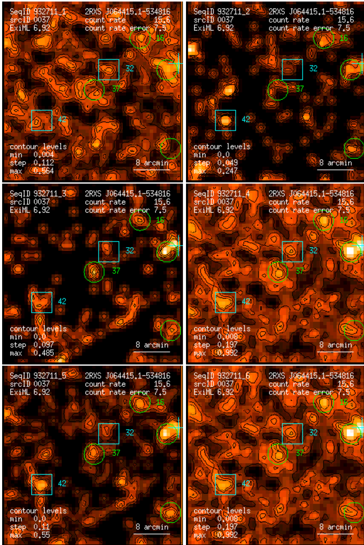
Figure 37: RASS 932711: detection 0037: band rate images, Gaussian filter: (1) PSPC channels 11 – 41, (2) 52 – 90, (3) 91 – 201, (4) 11 – 235, (5) 52 – 201, (6) 11 – 201. Broad band rates in counts/ks. Band rate contour levels in counts/ks/arcmin 2 .
